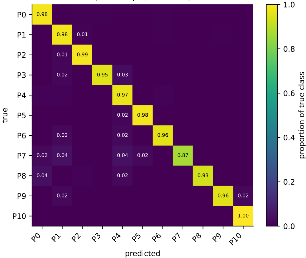
Confusion matrix — Gradient Boosting (random split, acc 96.6%)
