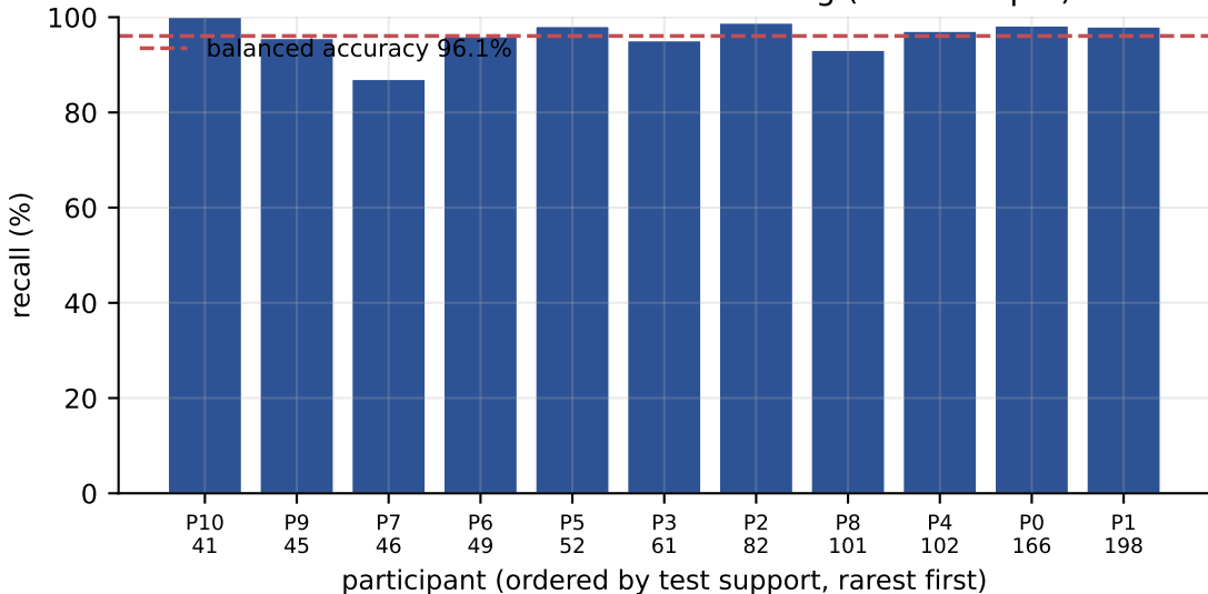
Per-class recall — Gradient Boosting (random split)
