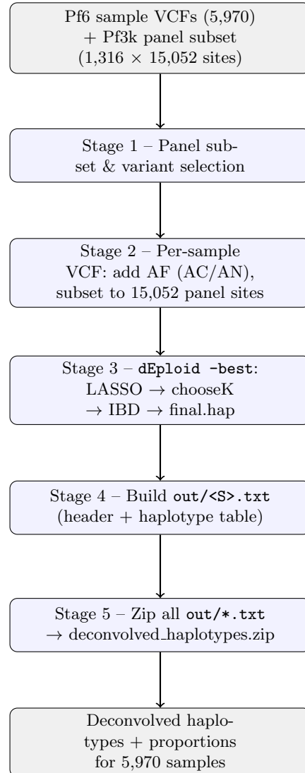
Figure S5.4: End-to-end DEploid-BEST field-sample deconvolution workflow. Each Pf6 sample VCF is intersected to the 15,052 panel sites and annotated with population allele frequency (AC/AN), then deconvolved by dEploid -best (LASSO panel shrinkage → strain-number selection → IBD haplotype/proportion inference → final haplotypes). Per-sample jobs run in parallel ( xargs -P 20 ) and the resulting haplotype tables are archived.
