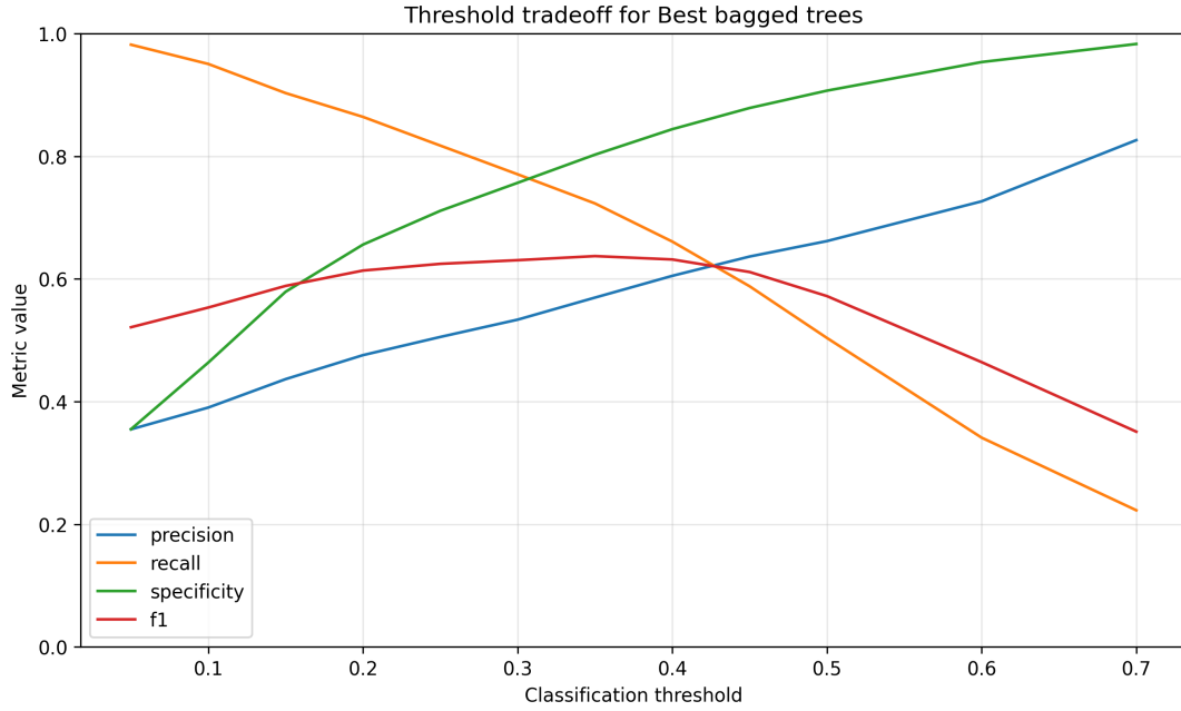
Figure 36: Threshold tradeoff for the selected bagged-tree ensemble
