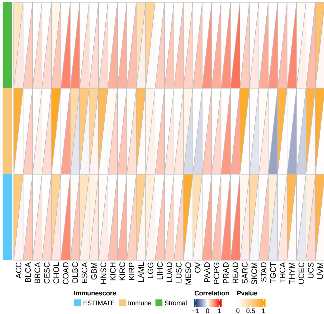
Correlation between TMEM45A and immunescores
