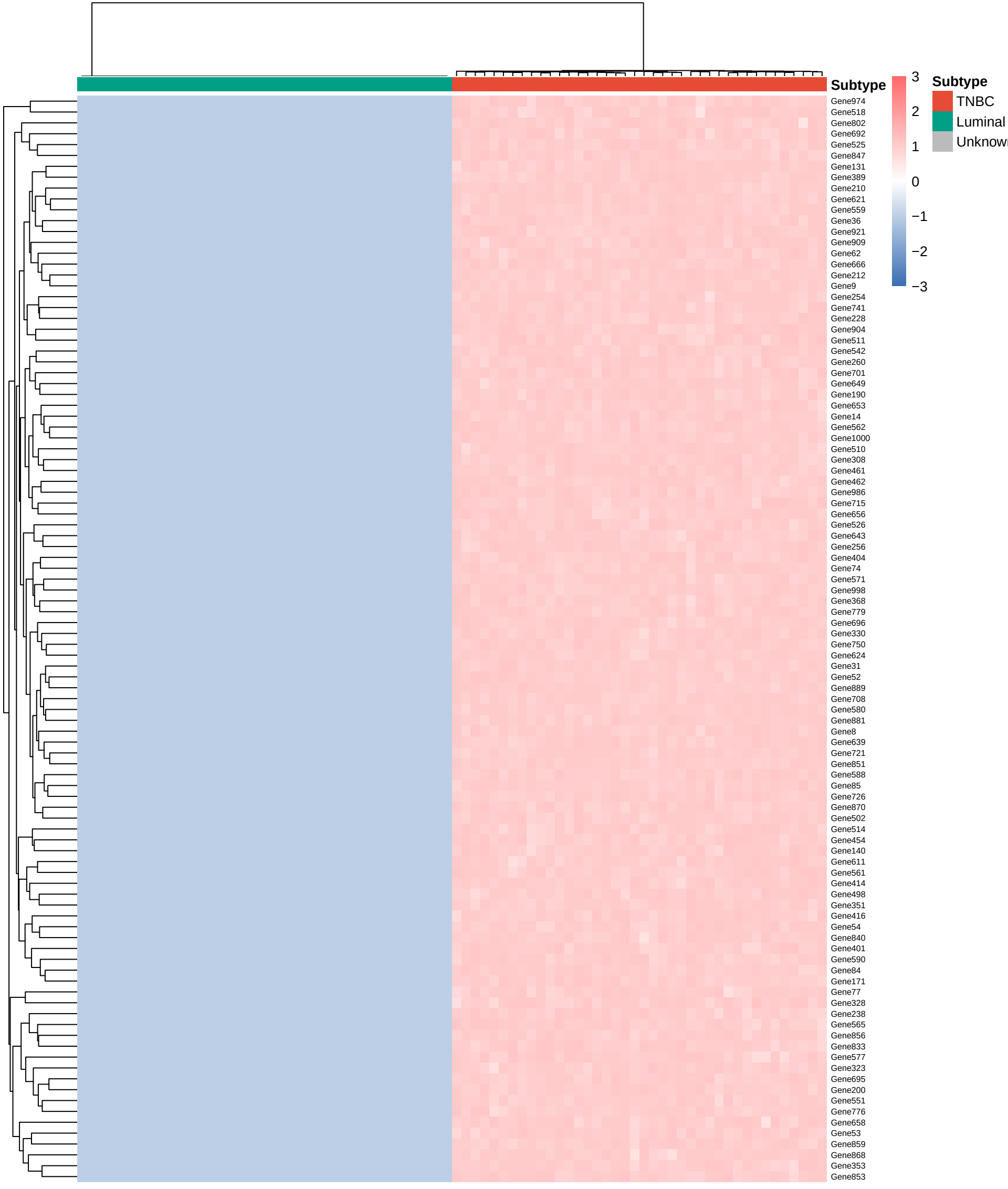
Top 100 DEG Expression Heatmap (Z-score VST)
