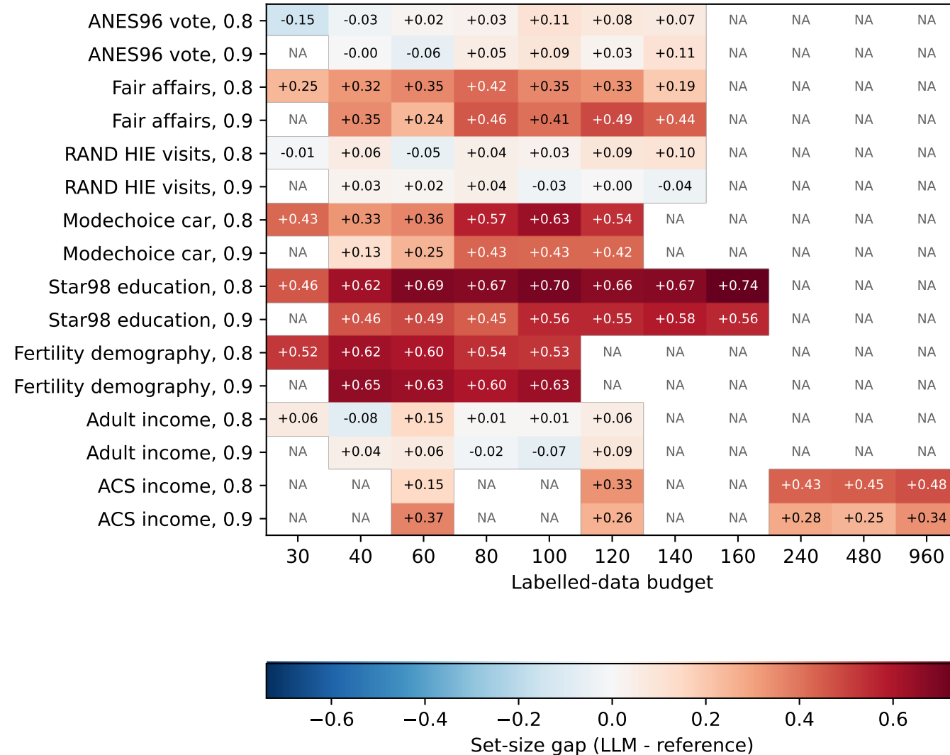
A LLM minus reference frontier set size
