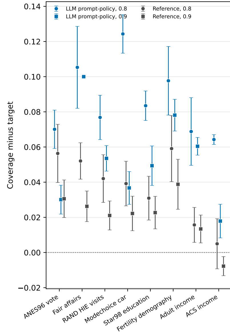
B Empirical coverage relative to target
