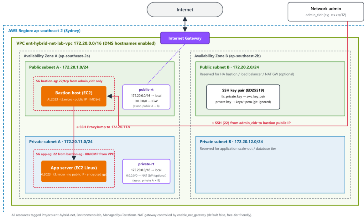
Figure 33: AWS architecture provisioned by Terraform (ap-southeast-2)
