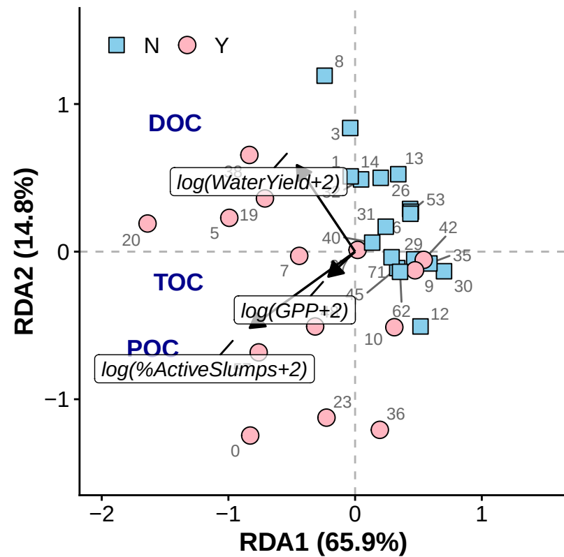
(a) R^2_{adj} = 78\%
