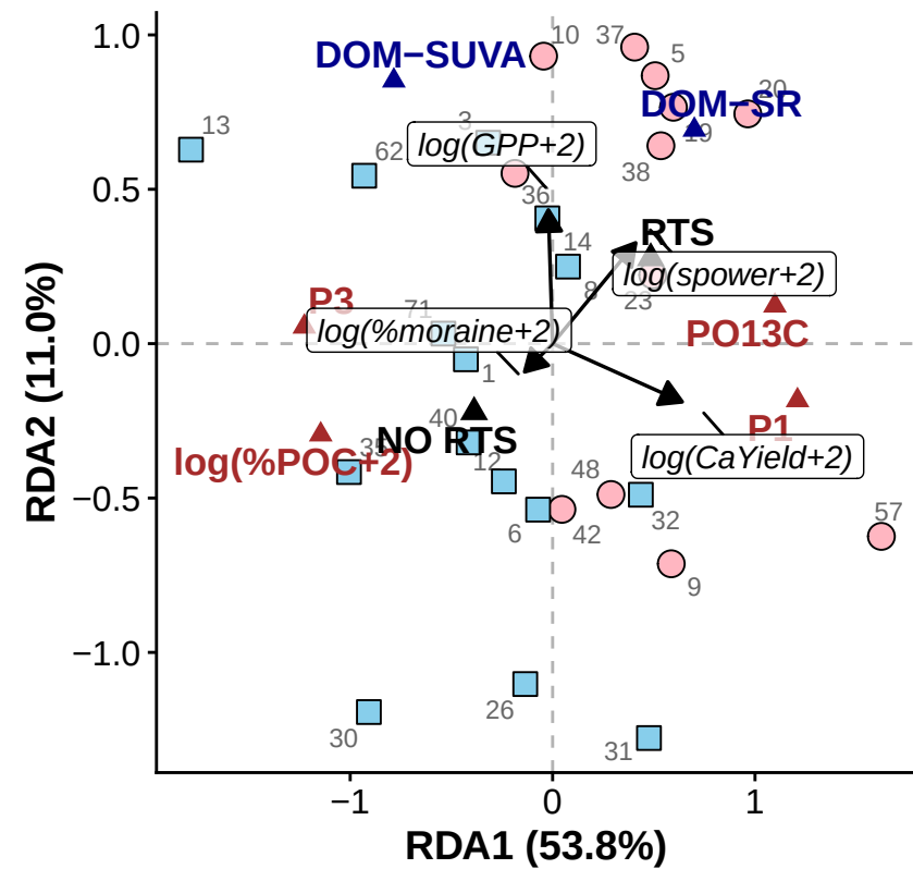
(c) R^2_{adj} = 62\%
