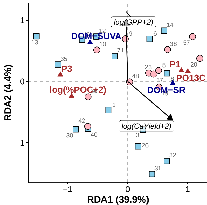
(b) R^2_{adj} = 40\%
