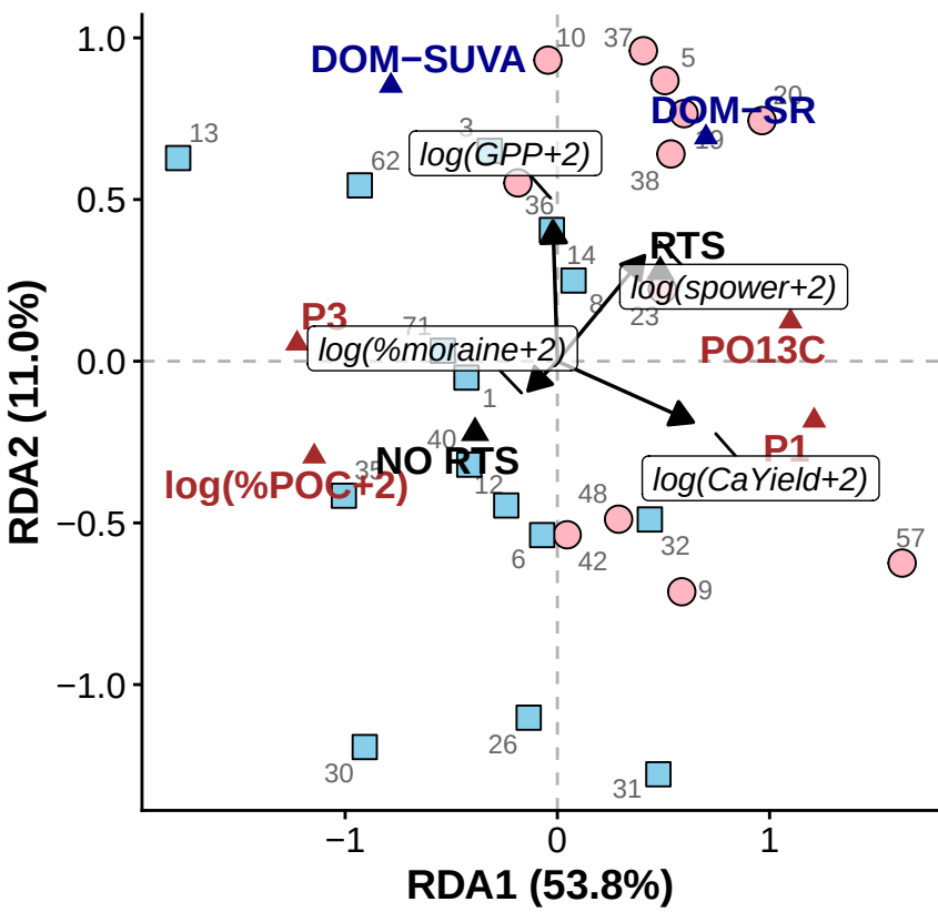
(c) R^2_{adj} = 62\%
