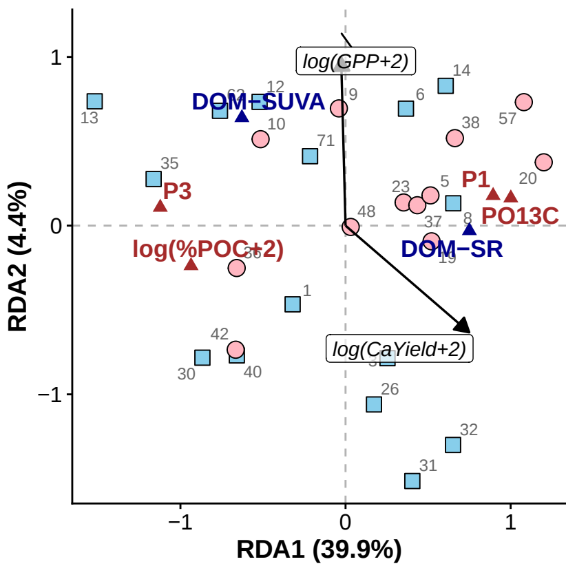
(b) R^2_{adj} = 40\%
