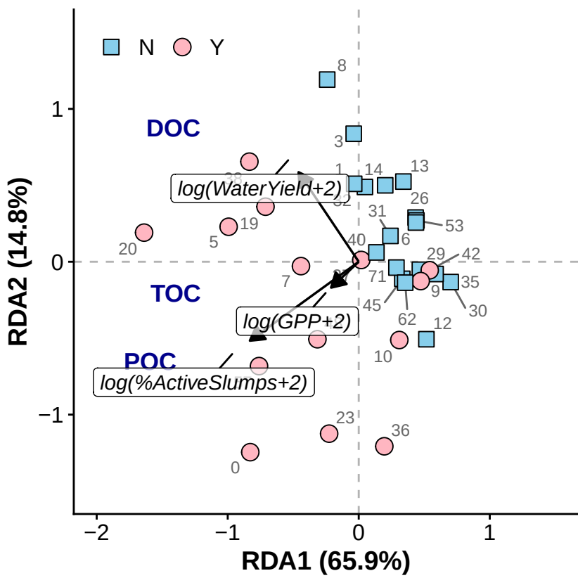
(a) R^2_{adj} = 78\%
