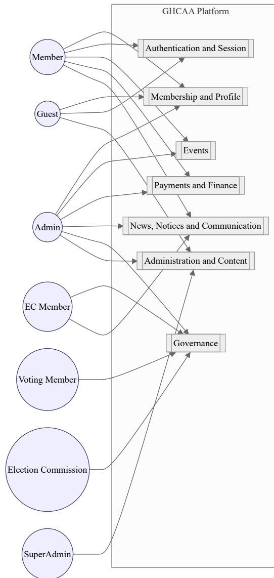
Fig. 3.1. System-level use-case diagram, packaged
