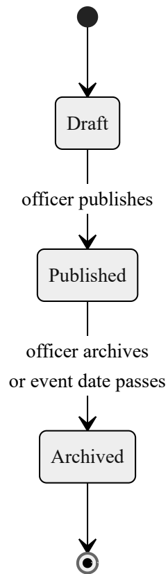
Fig. 5.14. State-machine diagram: event lifecycle
