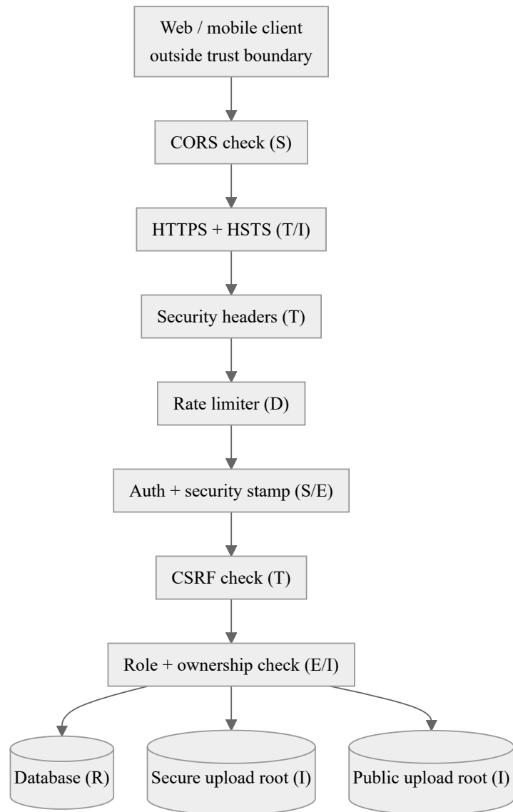
Fig. 8.1. Threat model data-flow diagram with trust boundaries, STRIDE-annotated
