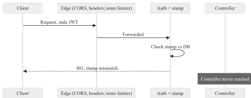
Fig. 8.5. Sequence diagram: an unauthorised request rejected through the middleware chain
