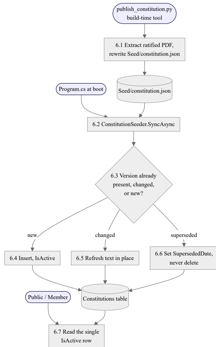
Fig. 5.5. DFD Level 2: Constitution publication
