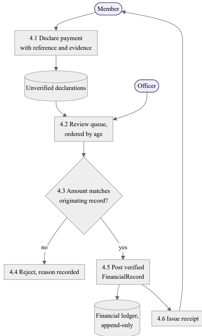
Fig. 5.3. DFD Level 2: Payment processing
