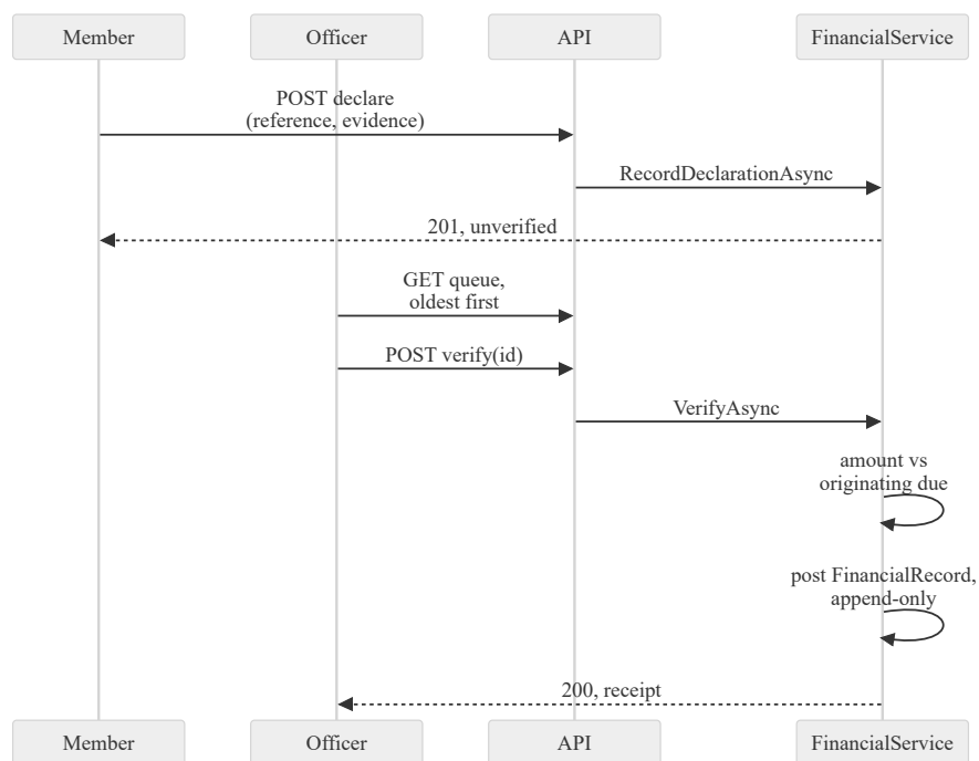
Fig. 5.17. Sequence diagram: payment declaration and verification
