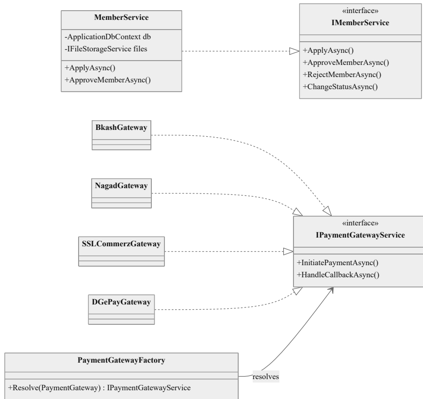
Fig. 6.8. Design class diagram: application interfaces and infrastructure services
