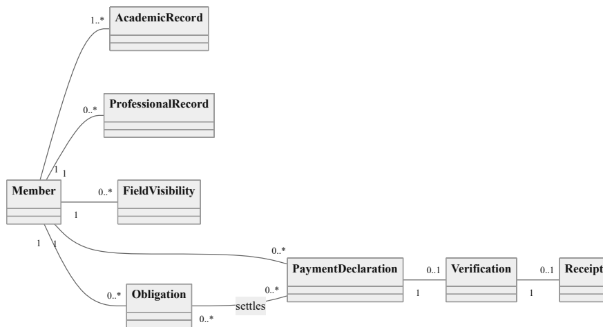
Fig. 3.8. Domain model, analysis level: membership, obligations and payment
