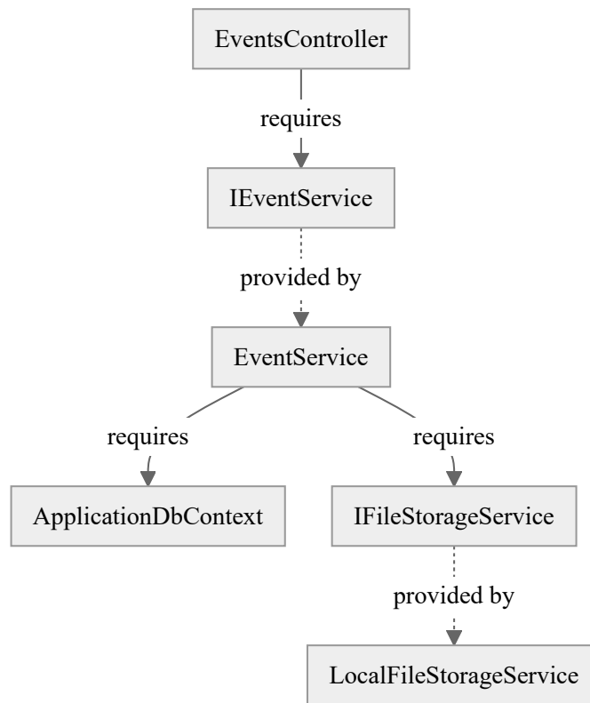
Fig. 6.9. Component diagram with provided and required interfaces
