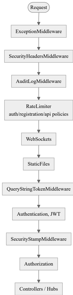
Fig. 6.10. Middleware pipeline diagram
