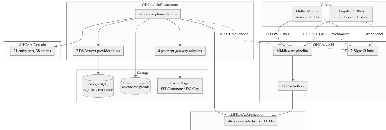
Fig. 6.1. High-level architecture diagram
