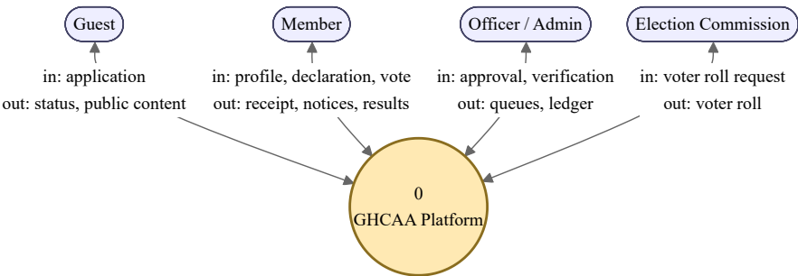
Fig. 5.1. DFD Level 0 (context). In and out are relative to the platform
