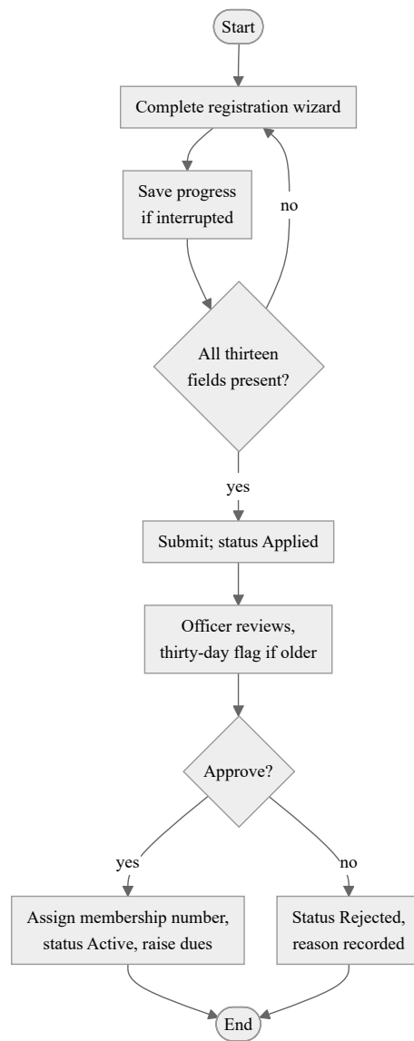
Fig. 5.6. Activity diagram: registration and administrative approval
