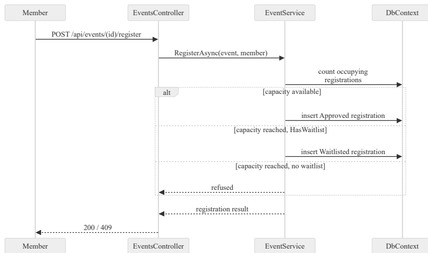
Fig. 5.16. Sequence diagram: event registration
