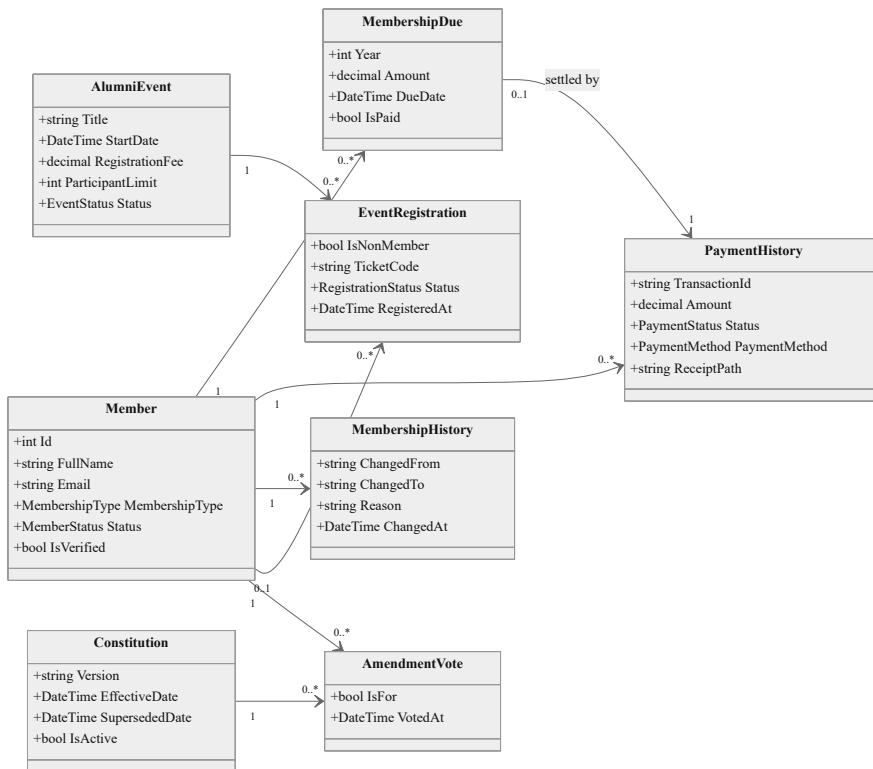
Fig. 6.7. Design class diagram: domain model
