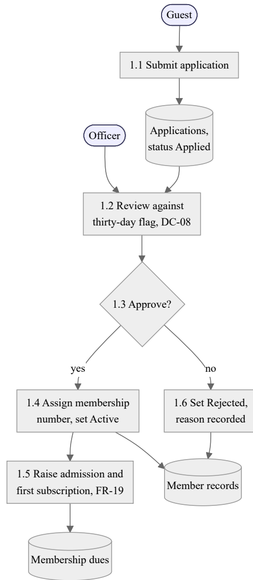
Fig. 5.4. DFD Level 2: Membership approval
