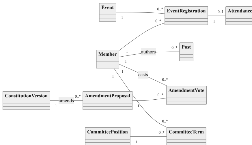
Fig. 3.9. Domain model, analysis level: participation, governance and content
