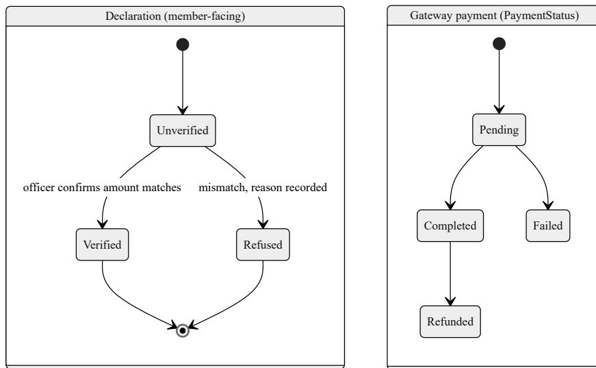
Fig. 5.12. State-machine diagram: payment and declaration
