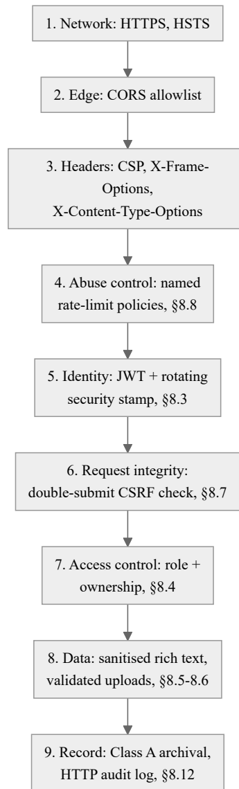
Fig. 8.6. Defence-in-depth layer diagram
