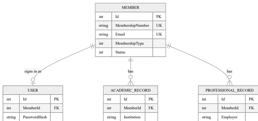
Fig. 6.3. Entity-relationship diagram, identity and records sub-model
