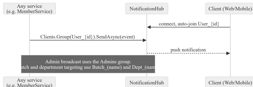
Fig. 5.18. Sequence diagram: real-time notification over SignalR
