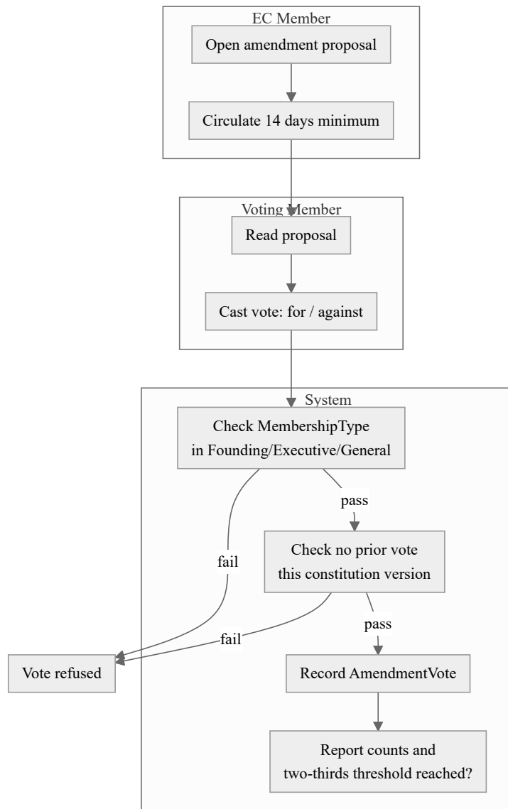
Fig. 5.9. Swimlane activity diagram: constitution amendment vote
