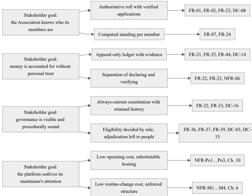
Fig. 3.12. Goal model
