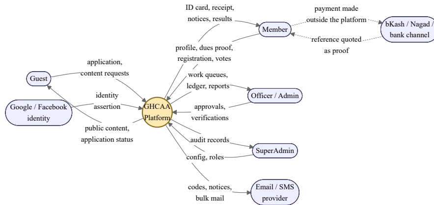
Fig. 1.1. Context diagram (DFD Level 0): platform boundary and external entities
