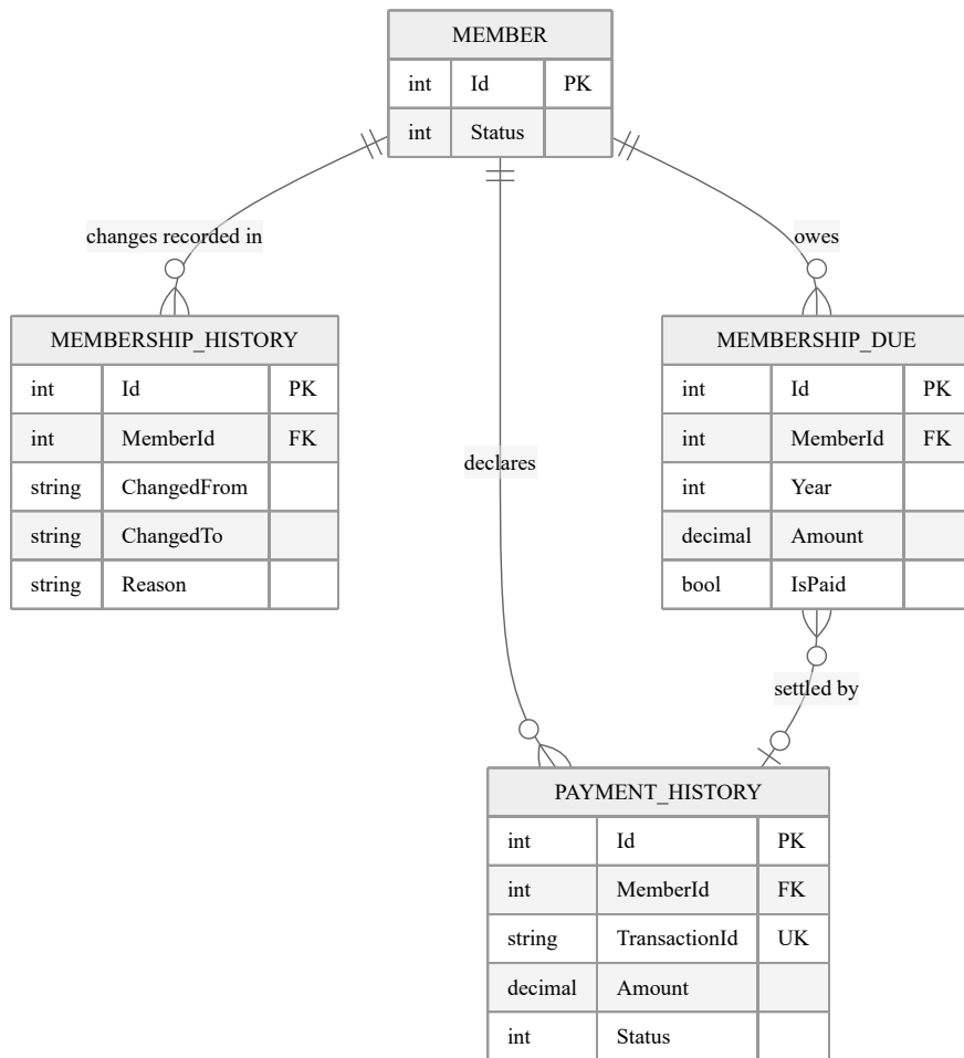
Fig. 6.4. Entity-relationship diagram, standing and money sub-model
