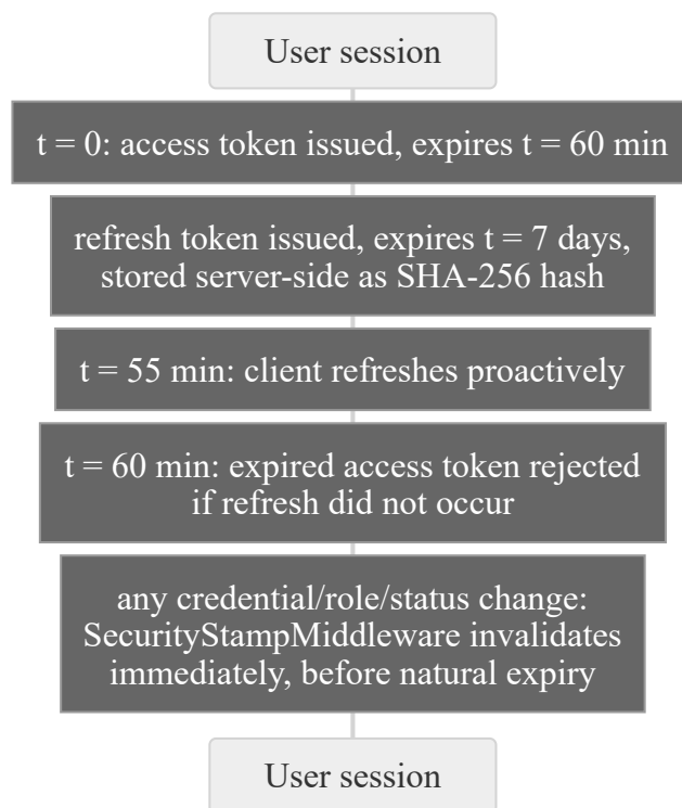
Fig. 5.19. Timing diagram: token lifetime and refresh window
