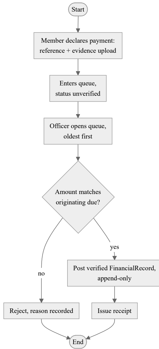
Fig. 5.7. Activity diagram: payment declaration and verification
