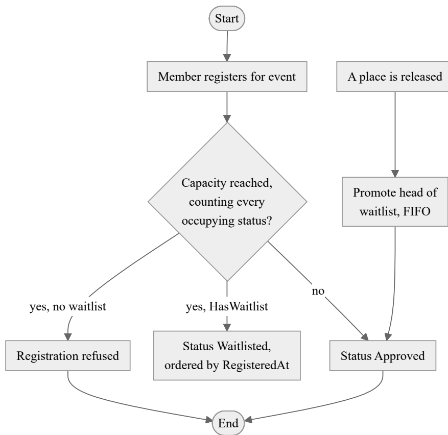
Fig. 5.8. Activity diagram: event registration with waitlist
