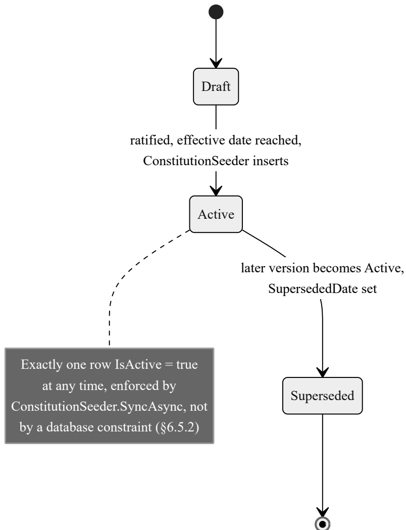
Fig. 5.13. State-machine diagram: constitution version
