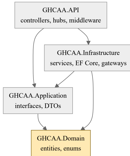
Fig. 6.2. Layered / clean architecture diagram with the dependency-inversion boundary marked
