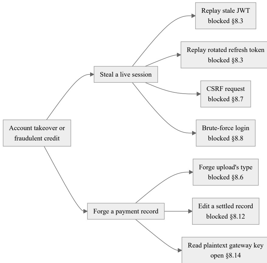
Fig. 8.2. Attack tree: member account takeover or fraudulent payment credit
