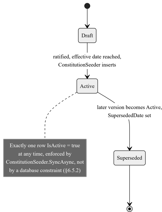
Fig. 5.13. State-machine diagram: constitution version
