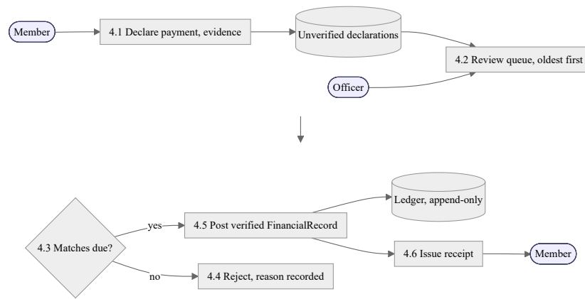
Fig. 5.3. DFD Level 2: Payment processing
