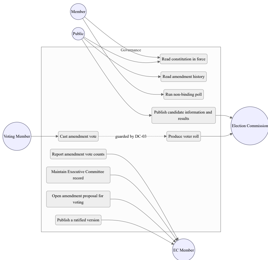
Fig. 3.5. Governance subsystem use cases
