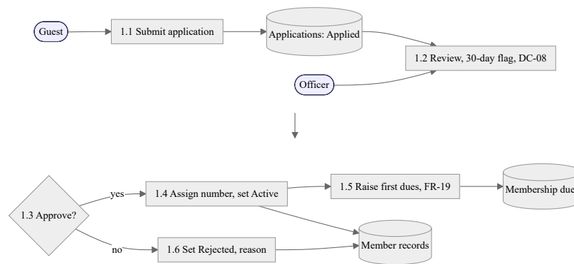
Fig. 5.4. DFD Level 2: Membership approval
