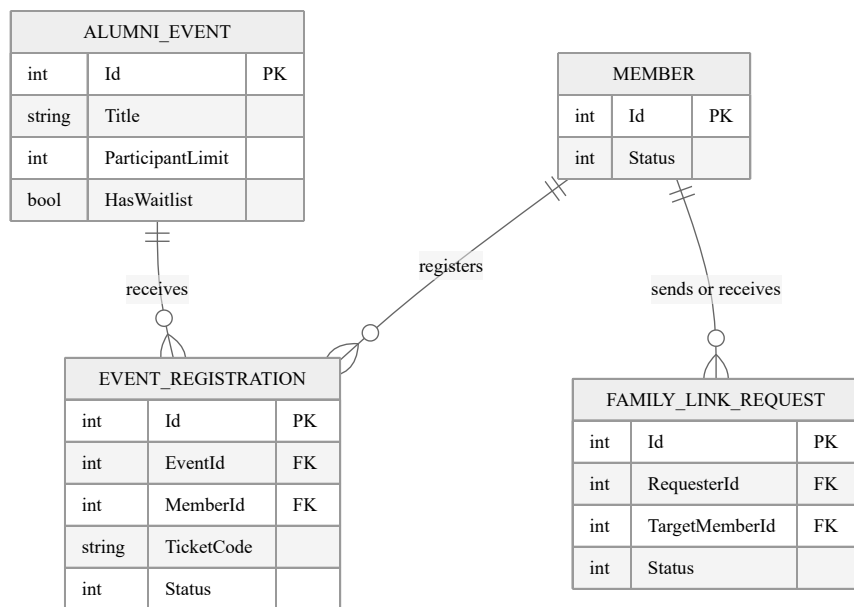
Fig. 6.5. Entity-relationship diagram, events and participation sub-model
