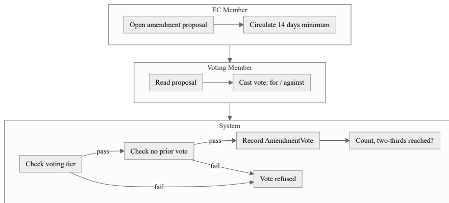
Fig. 5.9. Swimlane activity diagram: constitution amendment vote
