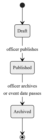
Fig. 5.14. State-machine diagram: event lifecycle
