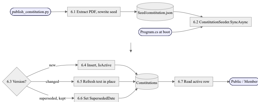
Fig. 5.5. DFD Level 2: Constitution publication
