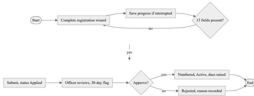
Fig. 5.6. Activity diagram: registration and administrative approval
