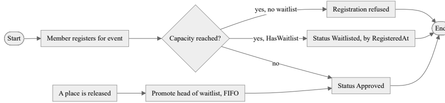
Fig. 5.8. Activity diagram: event registration with waitlist
