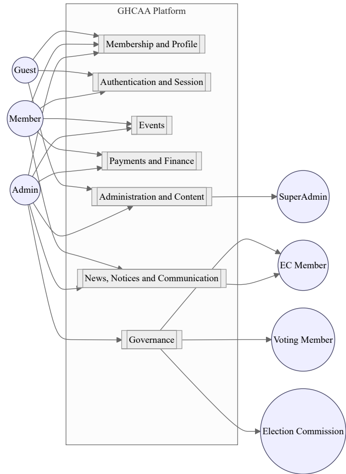
Fig. 3.1. System-level use-case diagram, packaged
