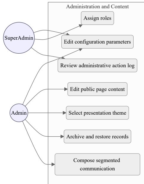
Fig. 3.6. Administration subsystem use cases
