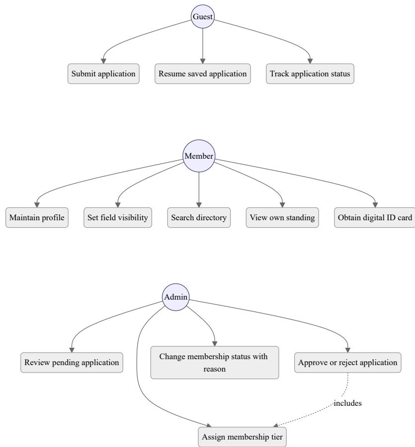
Fig. 3.2. Membership subsystem use cases
