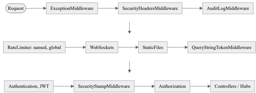
Fig. 6.10. Middleware pipeline diagram
