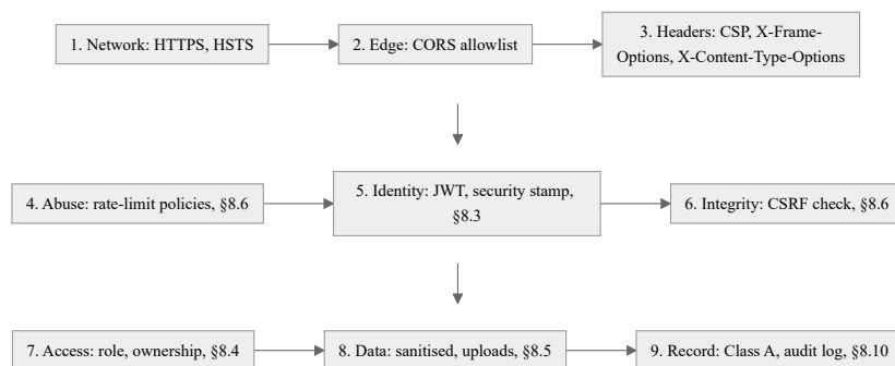
Fig. 8.6. Defence-in-depth layer diagram
