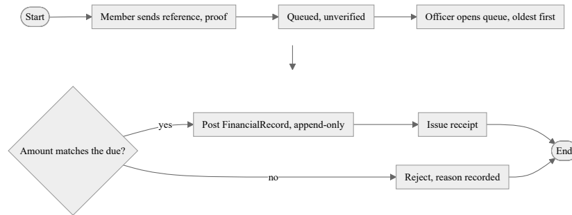
Fig. 5.7. Activity diagram: payment declaration and verification
