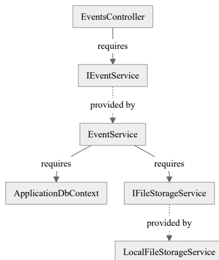
Fig. 6.9. Component diagram with provided and required interfaces
