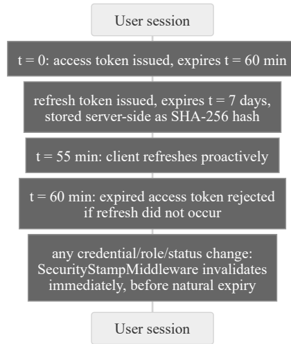
Fig. 5.19. Timing diagram: token lifetime and refresh window
