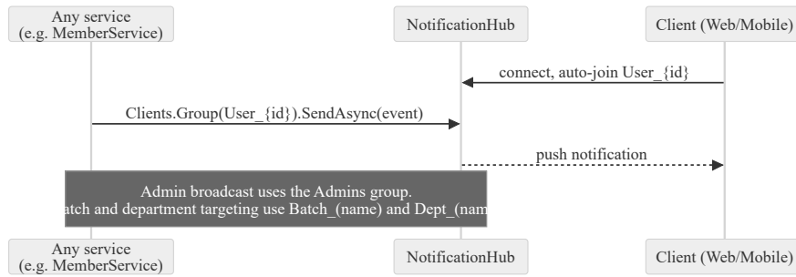
Fig. 5.18. Sequence diagram: real-time notification over SignalR
