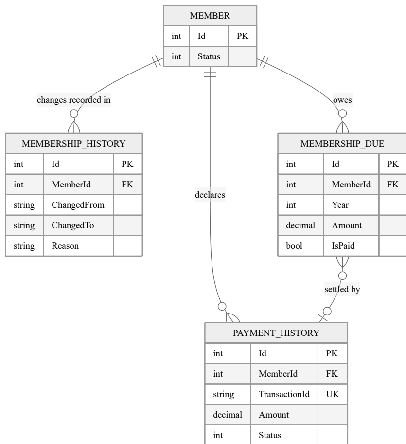
Fig. 6.4. Entity-relationship diagram, standing and money sub-model
