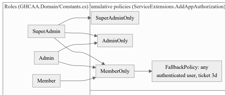
Fig. 8.3. Role-permission matrix diagram
