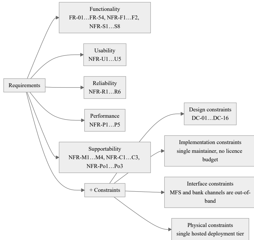
Fig. 3.11. Requirements classification, FURPS+
