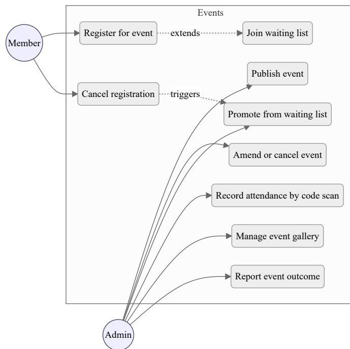
Fig. 3.3. Events subsystem use cases
