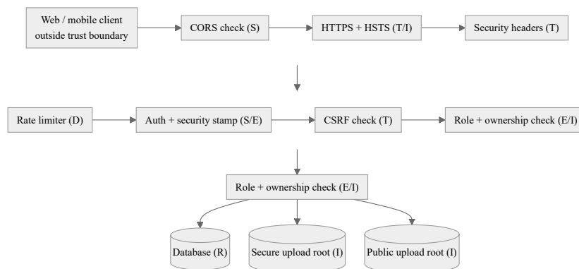
Fig. 8.1. Threat model data-flow diagram with trust boundaries, STRIDE-annotated
