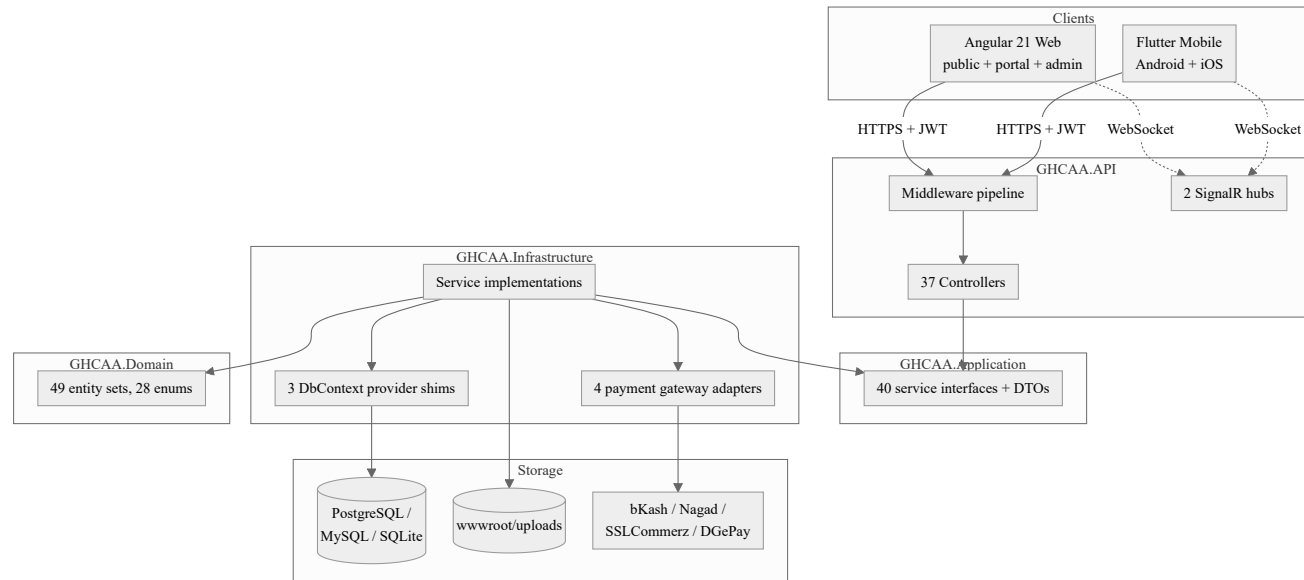
Fig. 6.1. High-level architecture diagram
