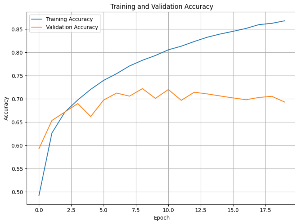
Figure 11: Training Accuracy and Validation Accuracy over Epochs
