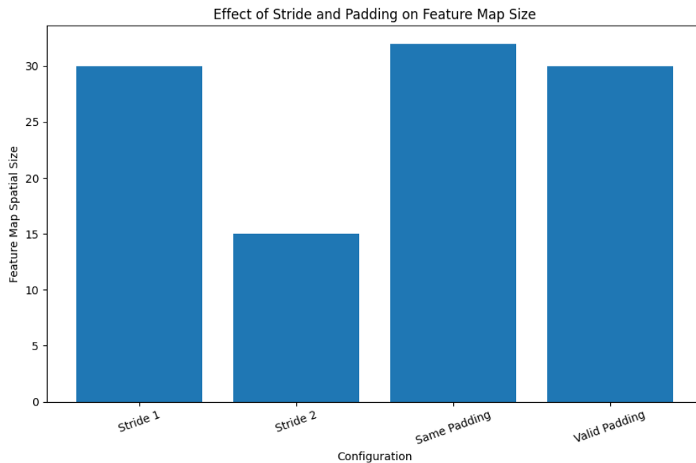
Figure 5: Comparison of stride and padding
