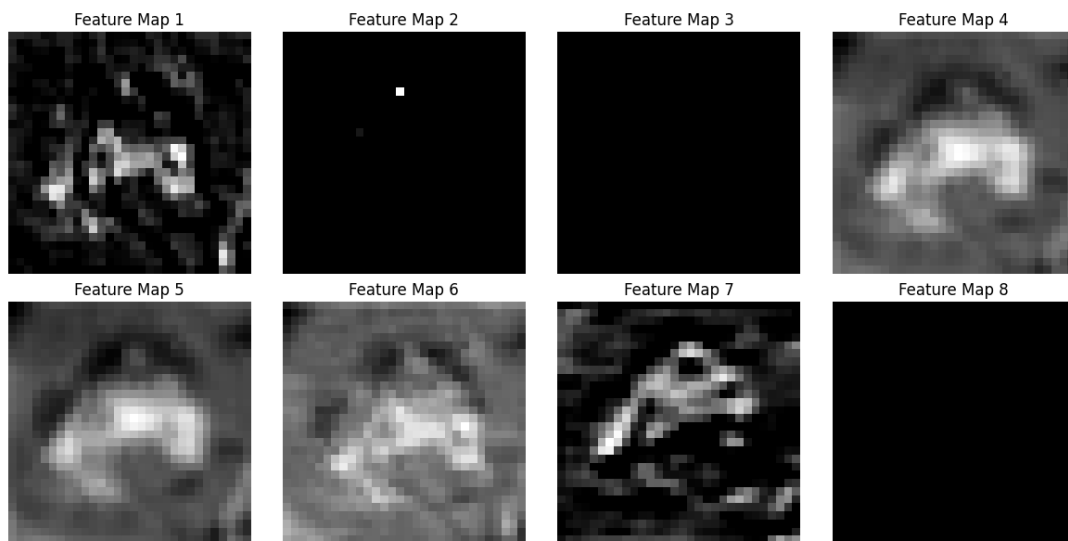
Figure 13: Feature Maps After First Convolution Layer
