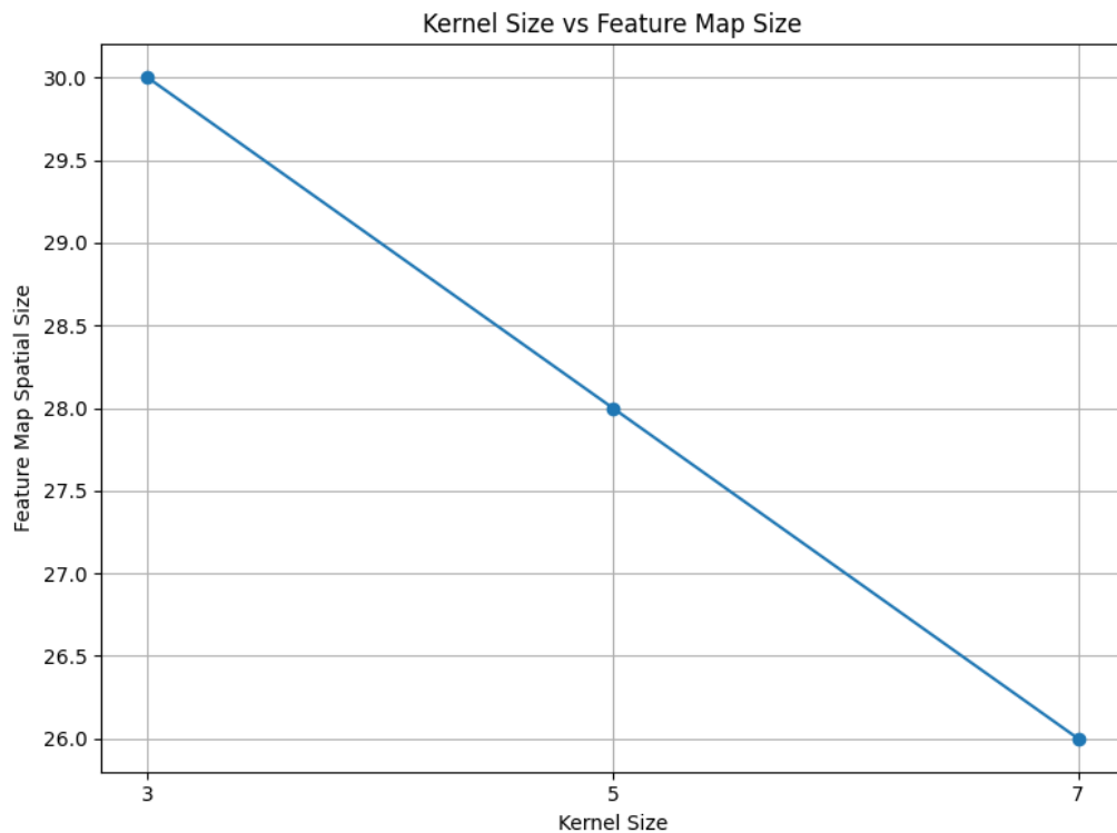
Figure 4: Comparison of kernel size and feature map size
