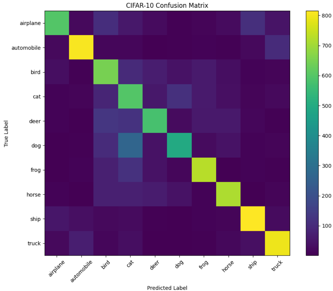
Figure 14: Confusion Matrix for CIFAR-10 Test Set
