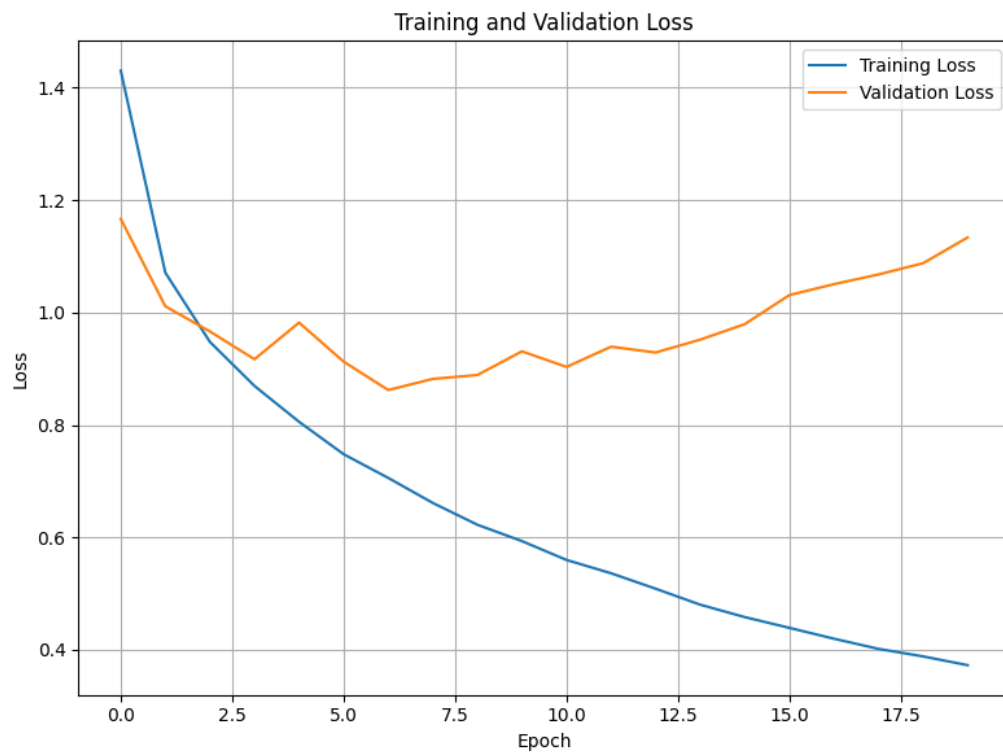
Figure 12: Training Loss and Validation Loss over Epochs
