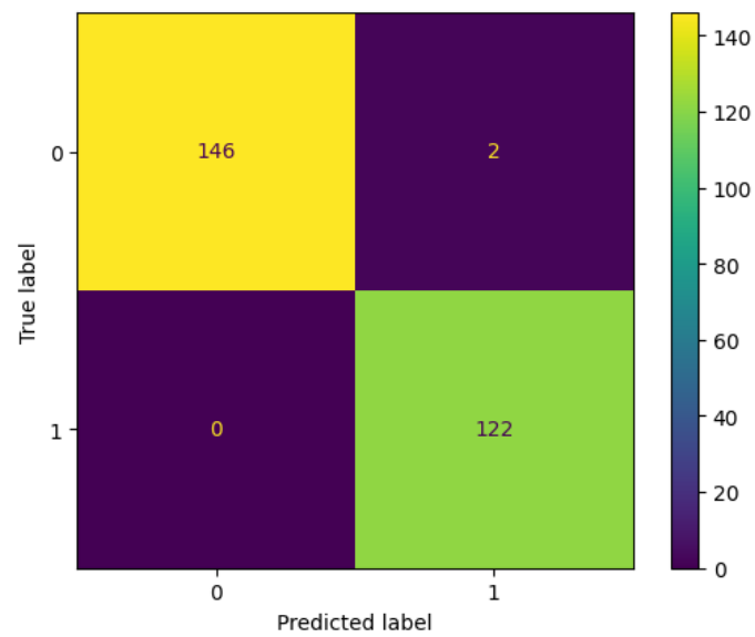
Figure 7: Confusion Matrix
