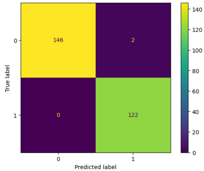
Figure 7: Confusion Matrix
