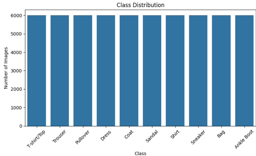
Figure 2: Class Distribution
