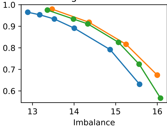
congress-bills 23
