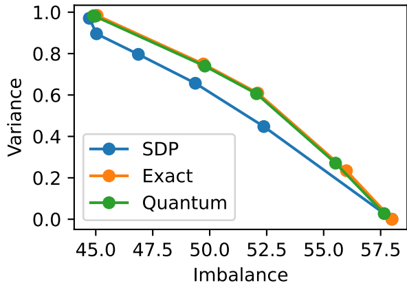
email-Enron 5
