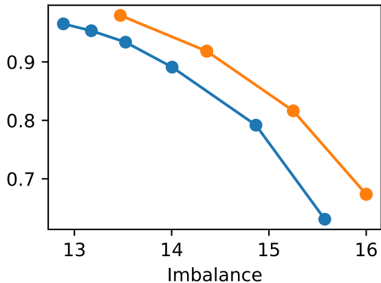
congress-bills 23
