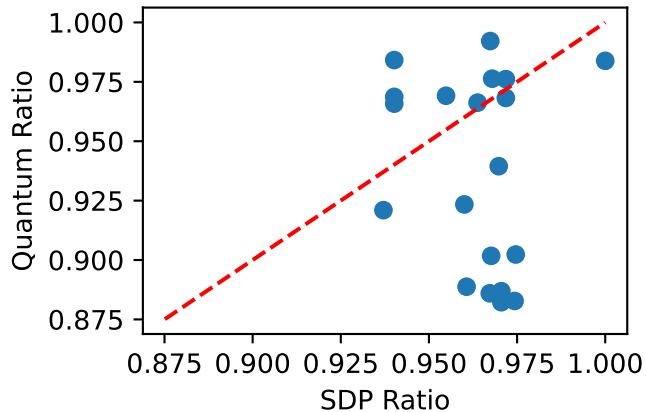
contact-high-school
