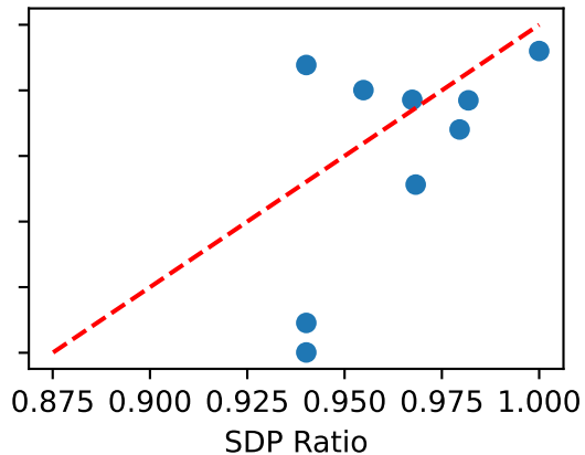
email-Enron
