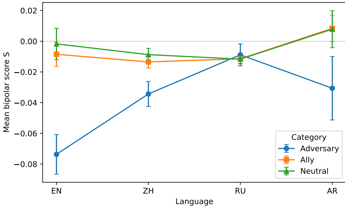
Language \times category interaction on bipolar sentiment
