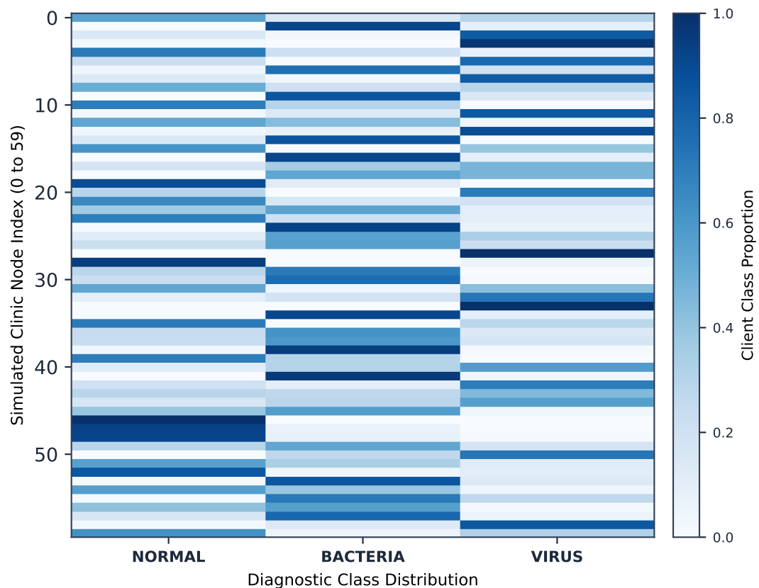
Figure 2. Patient-level dataset partitioning and non-IID distribution across 60 simulated clinic nodes.
