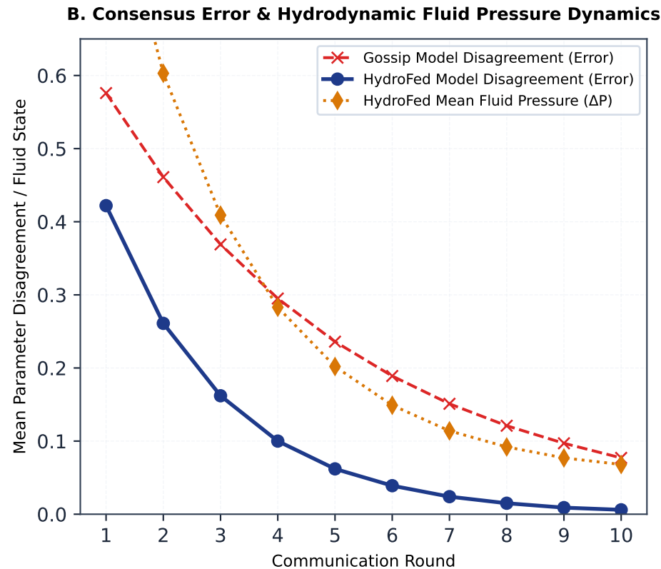
Figure 4. Federated learning convergence of the proposed HydroFed-ICAF consensus mechanism under non-IID clinic distributions.
