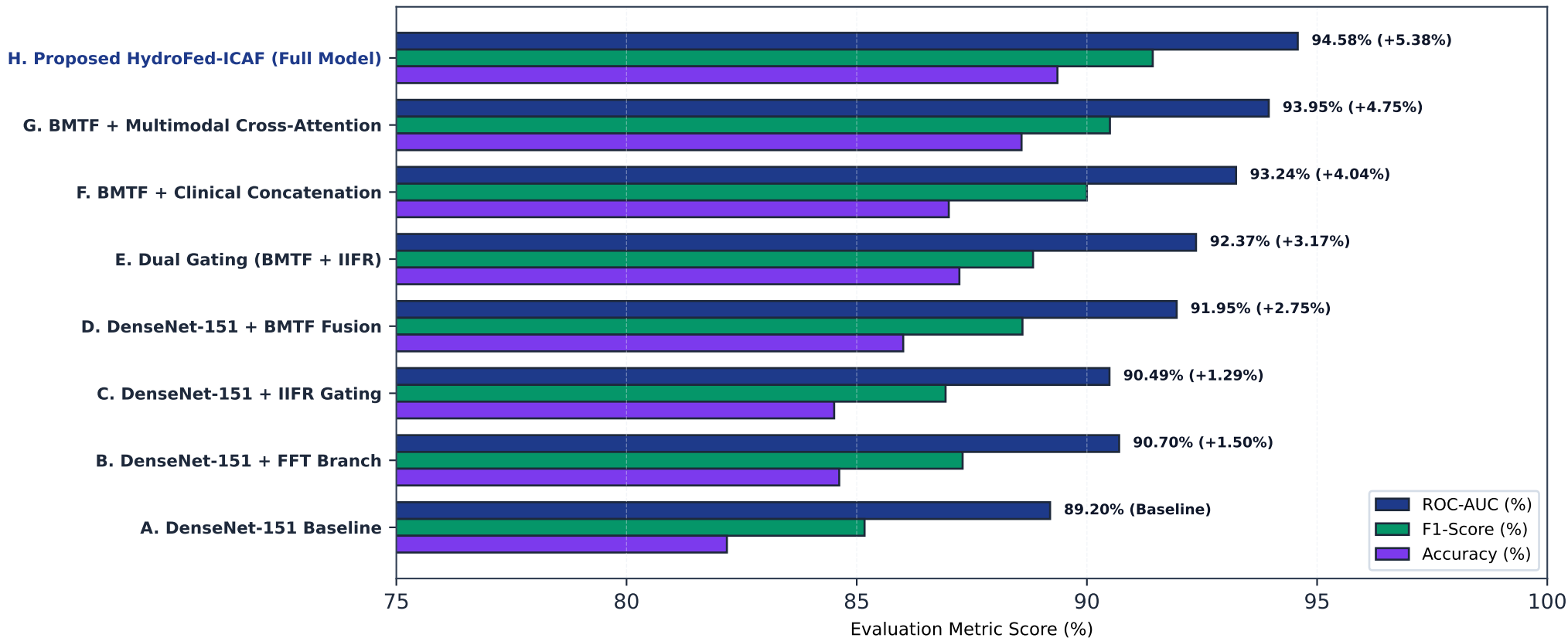
Figure 5. Ablation analysis of spatial, frequency-domain, immune-inspired, gating, and clinical cross-attention components.
