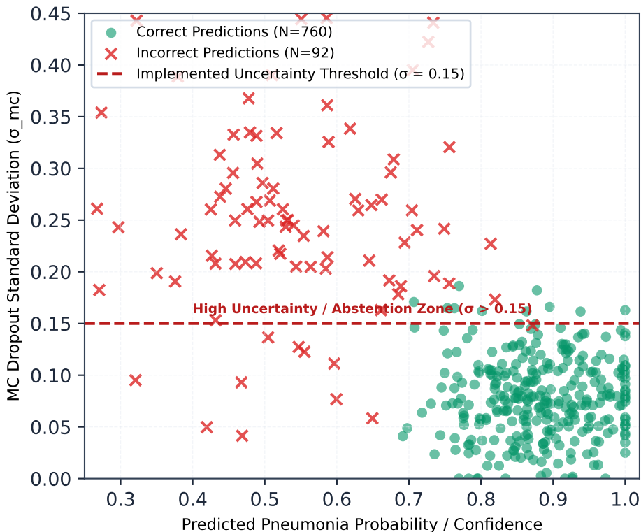
Figure 9. Prediction uncertainty estimated using 15 Monte Carlo dropout passes.
