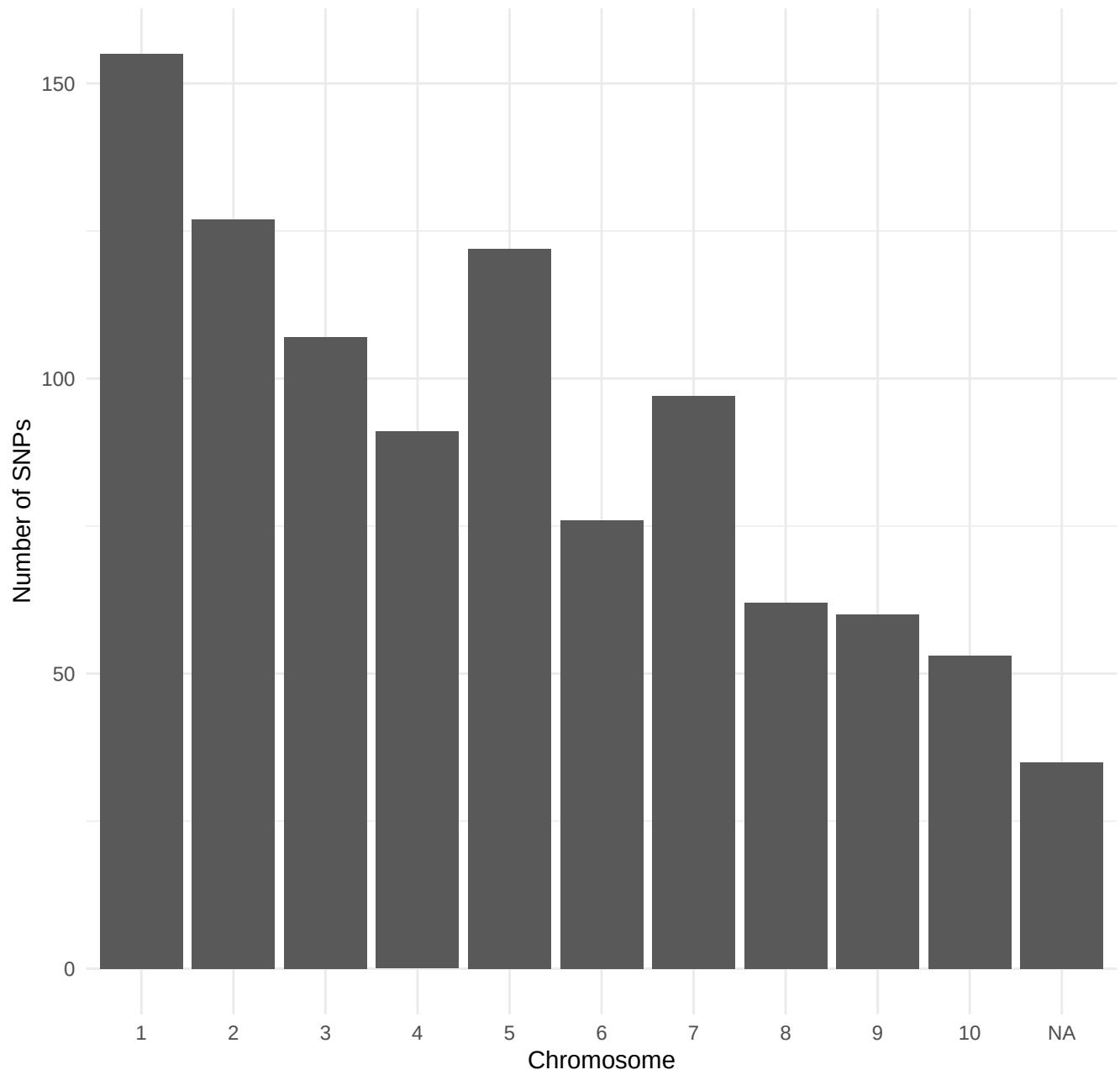
SNP Distribution
