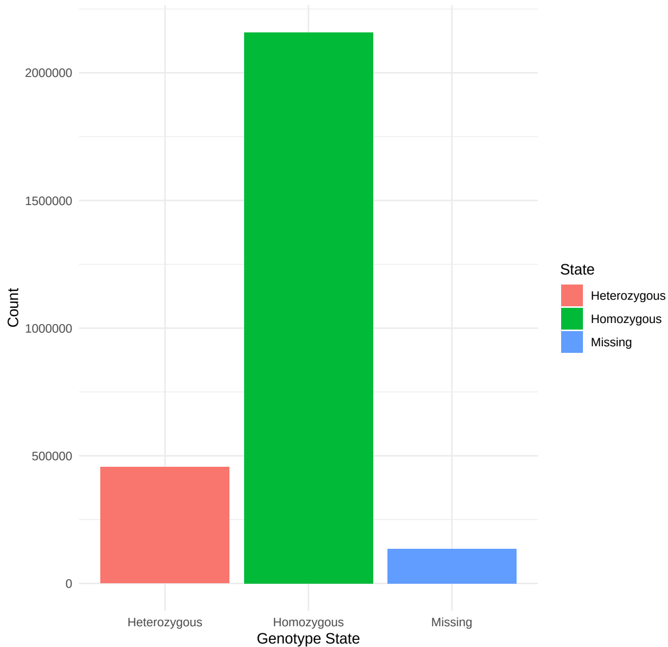
Overall Proportion of Homozygous, Heterozygous, and Missing Data
