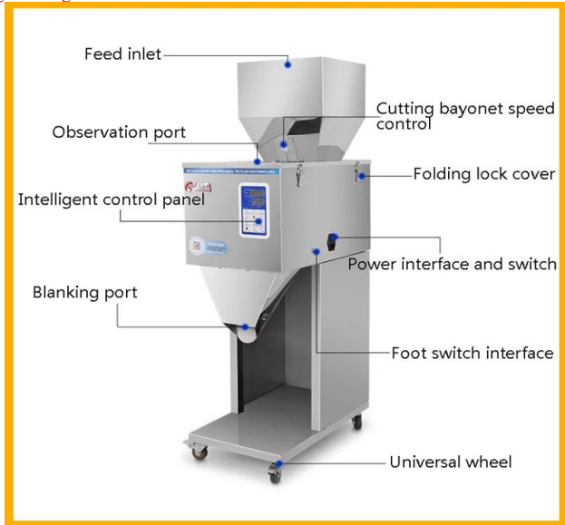
Semi auto-Digital program weight filling machine 200-2000gm.
