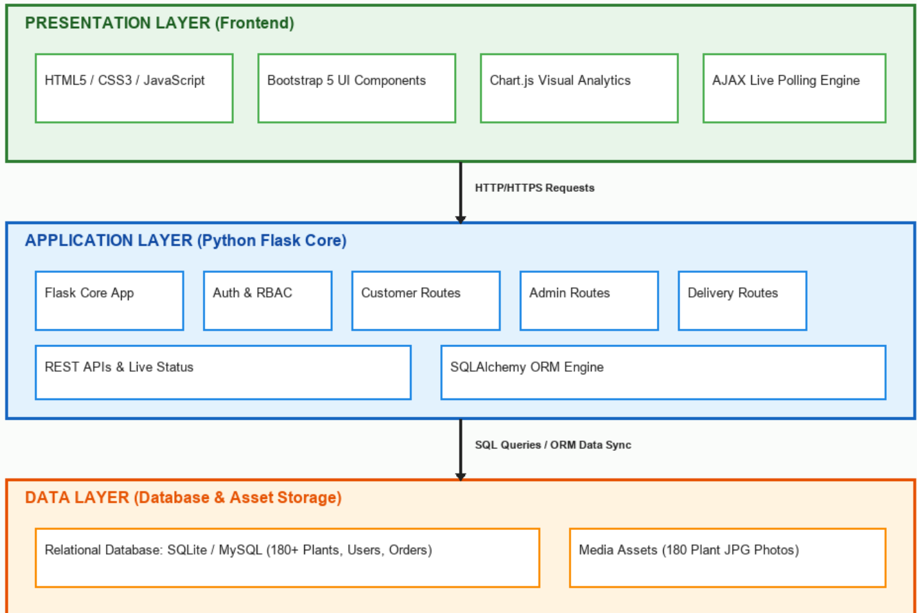
GreenCart - 3-Tier System Block Diagram
