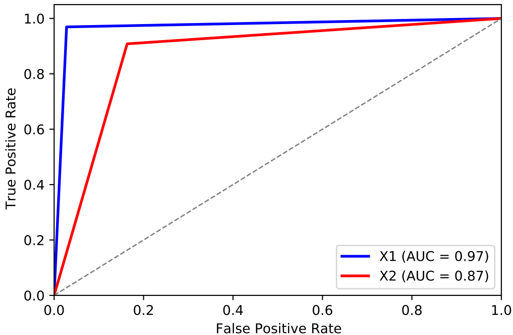
ROC Curve for Decision Tree Classifiers
