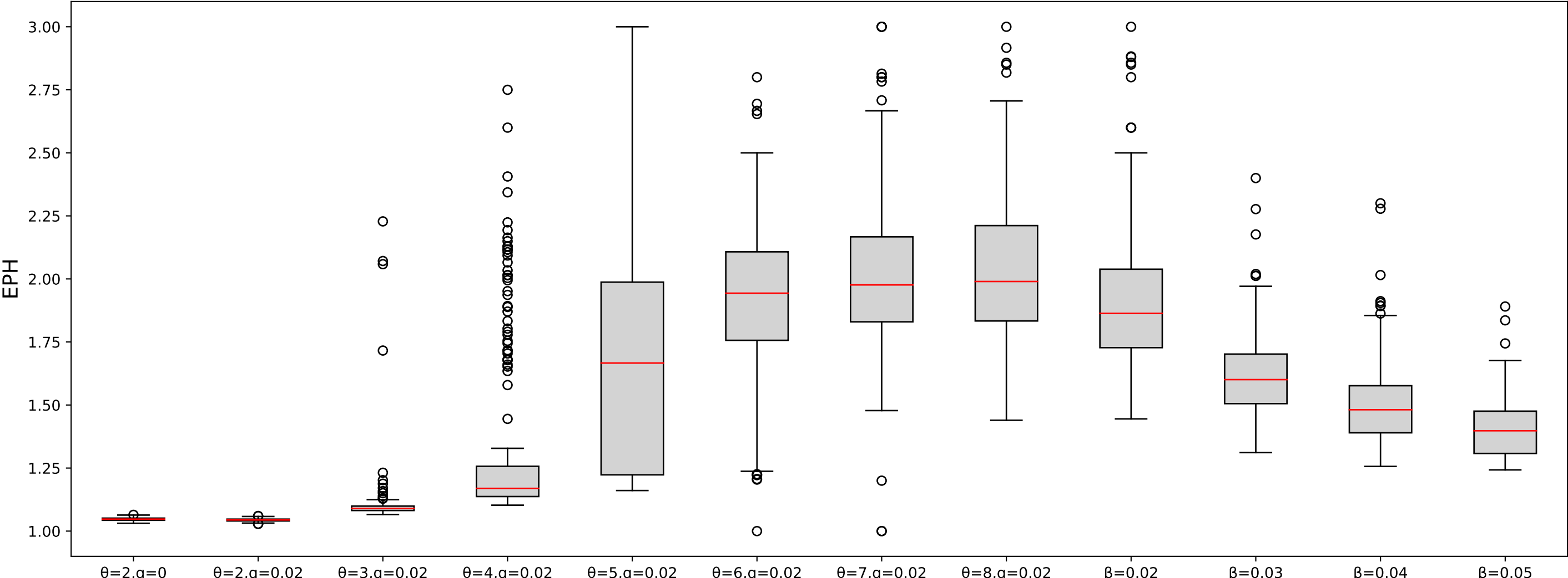
Box Plot of EPH Distributions
