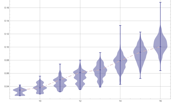
(B) Some knots from 9 to 16 crossings, using contraction sequences of width 6.
