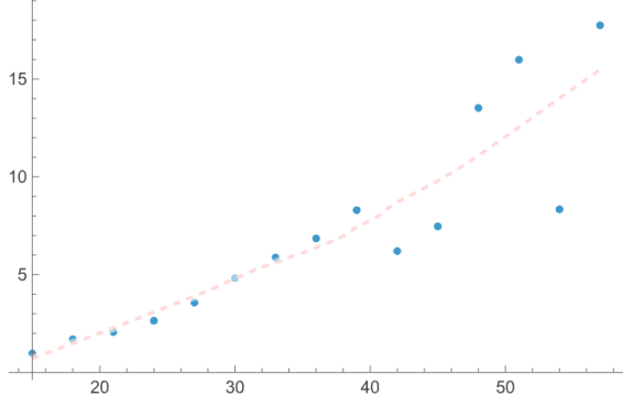
(C) (3, i) -torus links with i = 6, \dots, 20 , all using contraction sequences of width 8.
