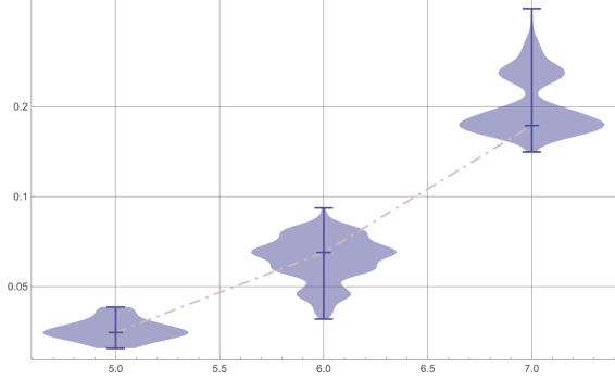
(A) The first 2000 knots with 13 crossings in the knot table [HTW98], plotted in log scale.
