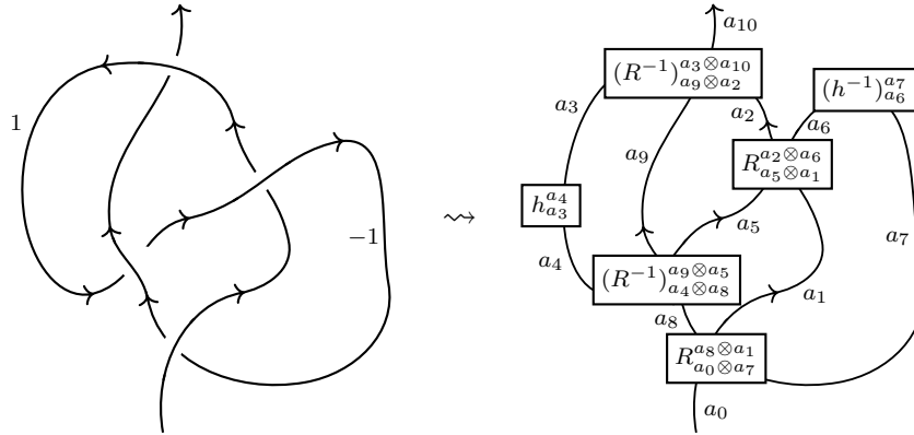
FIGURE 3. The tensor network resulting from an oriented long knot diagram of the 4_1 knot.
