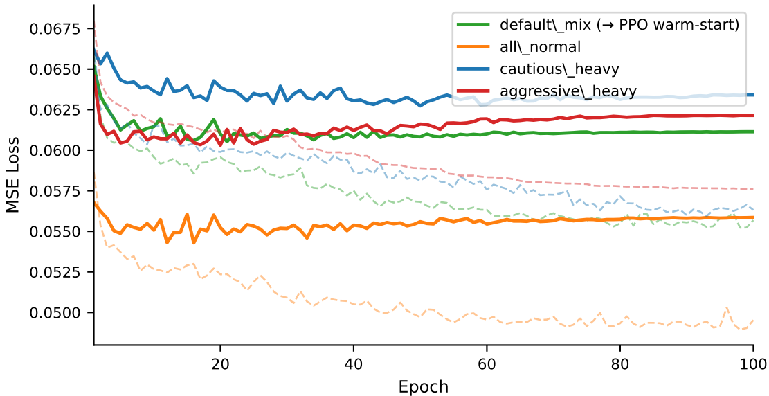
BC training and validation loss (solid = val, dashed = train)
