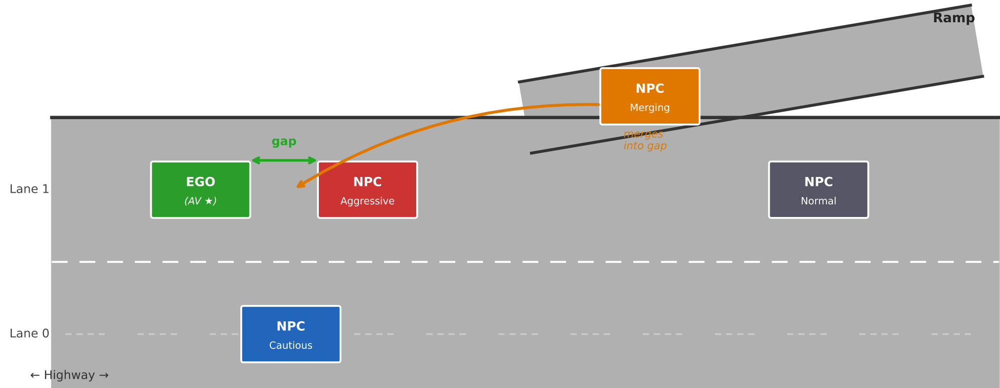
Highway-Env merge-v0 — ego manages gap while NPC merges from ramp Driver types randomly assigned each episode from {cautious, normal, aggressive}
