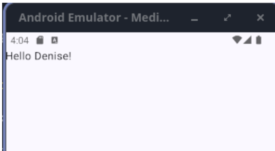
Figura 15: Hello Denise
