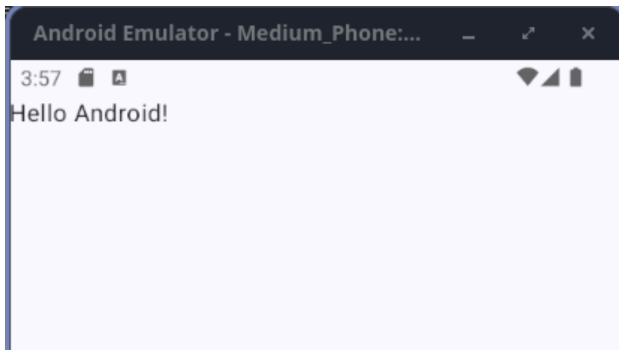
Figura 13: Hello Android
