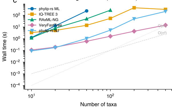
c Scaling behavior (1000 sites)
