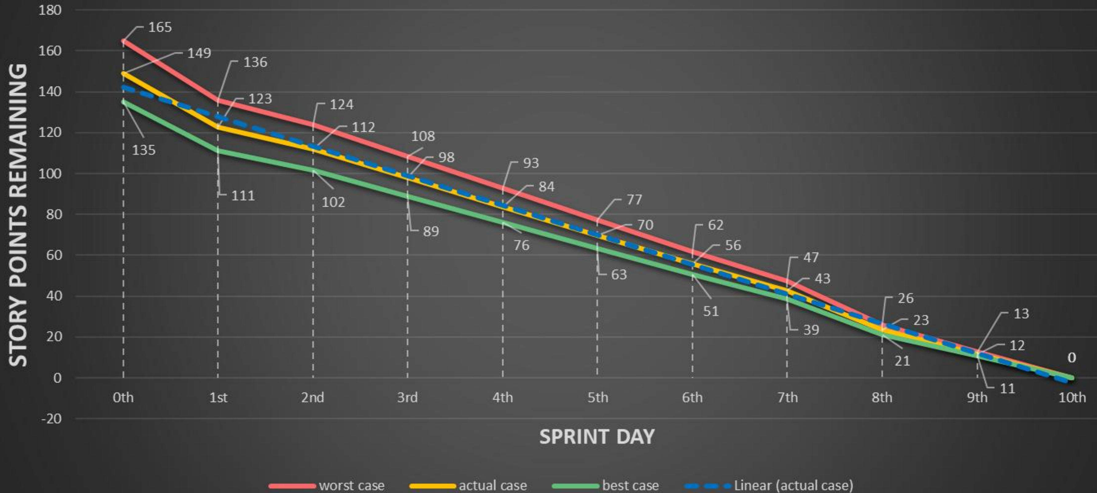
BURNDOWN CHART FOR SPRINT 2
