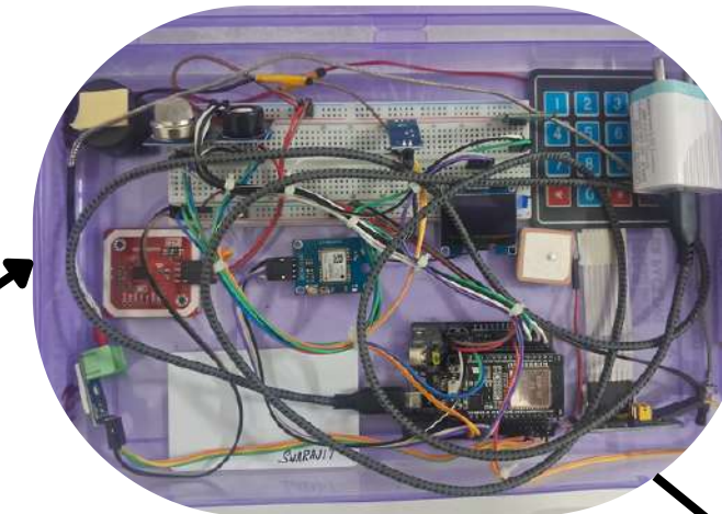
ESP32-Subsystem
