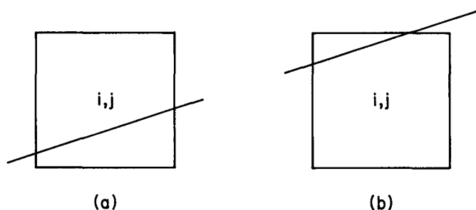
Fig. 3. Bresenham's error measure gives the same grey scale value as the fractional area of the pixel square (a) covered by the white side of the edge. In case (b), the error measure gives the appropriate shade of grey for smoothing the edge with a single pixel element, leaving the upper element completely black.
