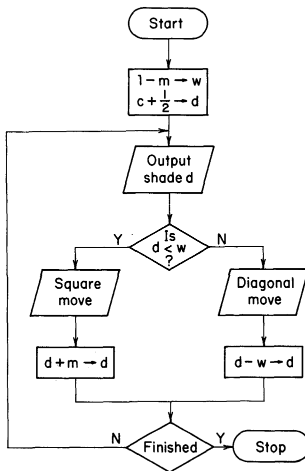
Fig. 1. A form of Bresenham's algorithm for the generation of the straight line y = mx + c , where 0 < m < 1 (first octant), and c < \frac{1}{2} (the origin is a sensible starting point). The algorithm has been modified so that d operates in the range 0 \leq d < 1 .
