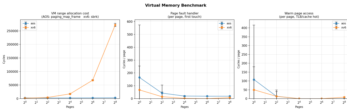
Figure 15: Results of virtual memory microbenchmarks.
