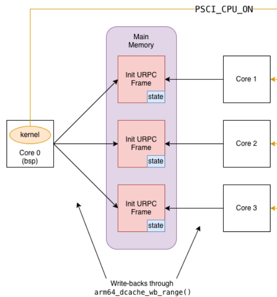
Figure 12: Multicore Architecture
