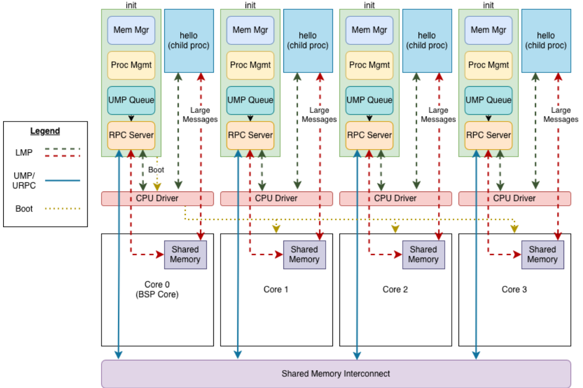
Figure 1: Core OS Architecture
