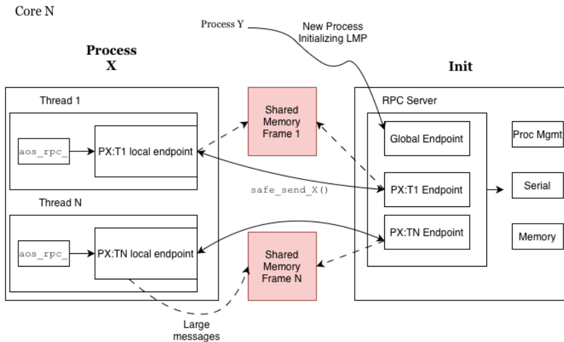
Figure 8: Overall LMP subsystem architecture.
