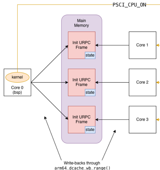
Figure 12: Multicore Architecture
