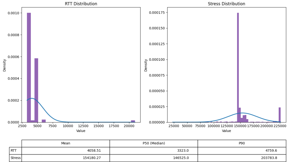
Figure 9: Per-thread implementation benchmark results for a single-threaded number passing benchmark, labeled RTT, and a multithreaded string passing benchmark, labeled stress. As can be seen the overhead to create a perthread channel (evident in the median RTT statistic) is negligible compared to the baseline. The per-thread implementation sees significant gains in median multithreaded latency.
