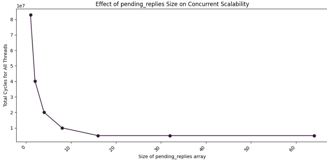
Figure 7: Results show linear speedup in the number of slots in pending_replies , until there are enough slots for each thread at which point there are no additional returns.
