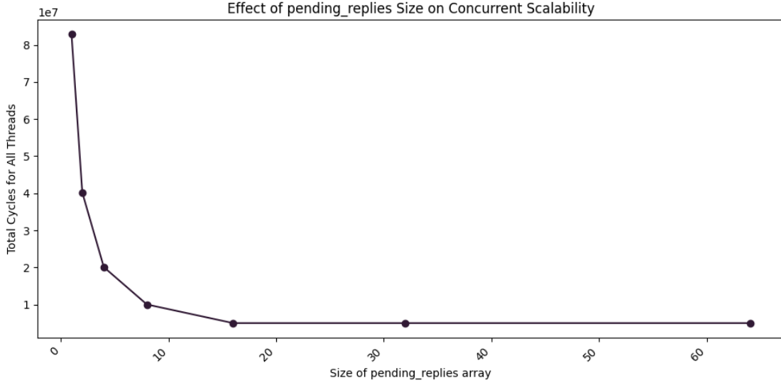
Figure 6: Performance scales linearly with the number of slots in pending_replies , until there are enough slots for each thread at which point there are no additional returns.
