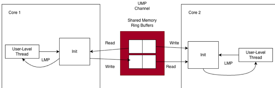
Figure 5: High-level overview of the RPC system.
