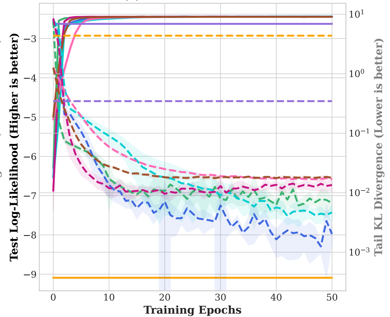
(c) Zero-Inflated NB
