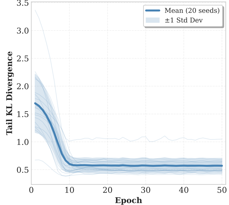
(c) Tail Learning Performance
