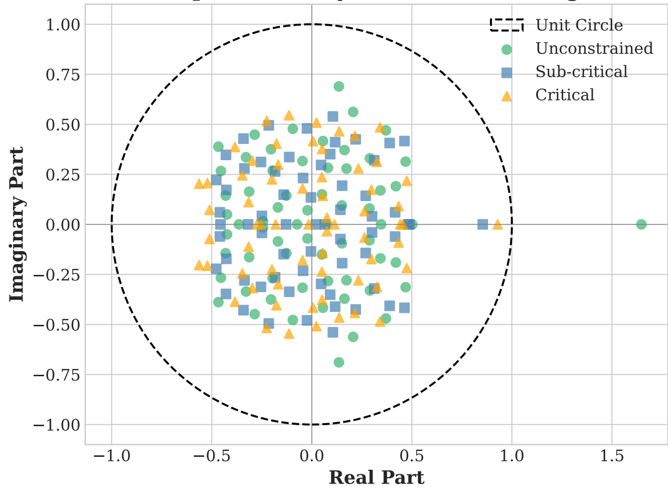
(b) Spectral Analysis of Learned Weights
