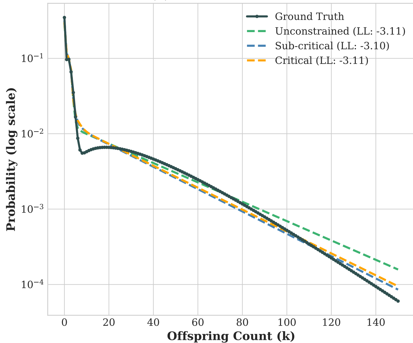
(a) Distributional Fits
