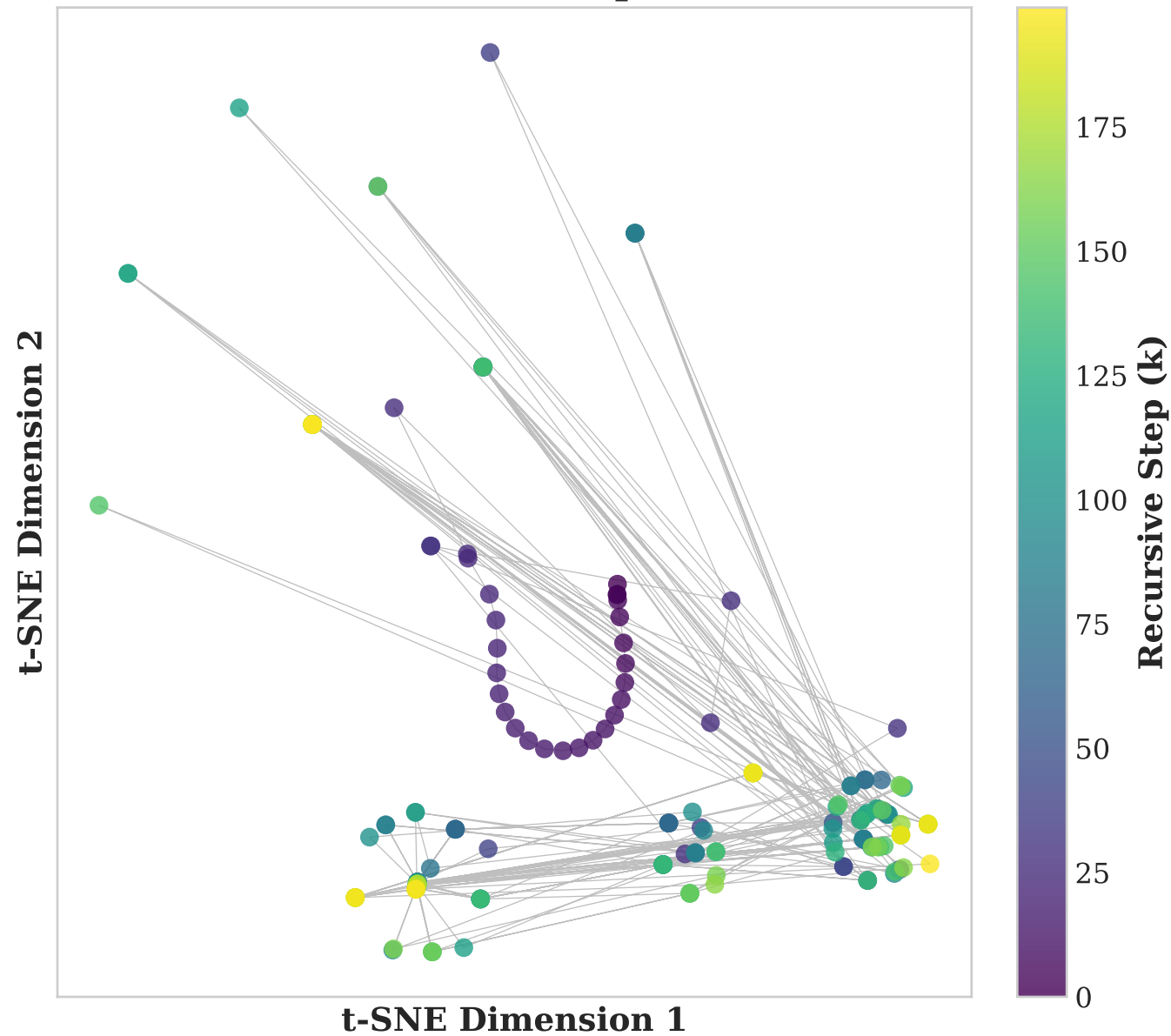
(a) The Learned State-Space Manifold
